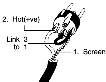
Unbalanced Mic XLR
