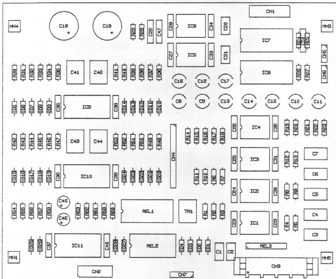
PAGE 17 analog board
