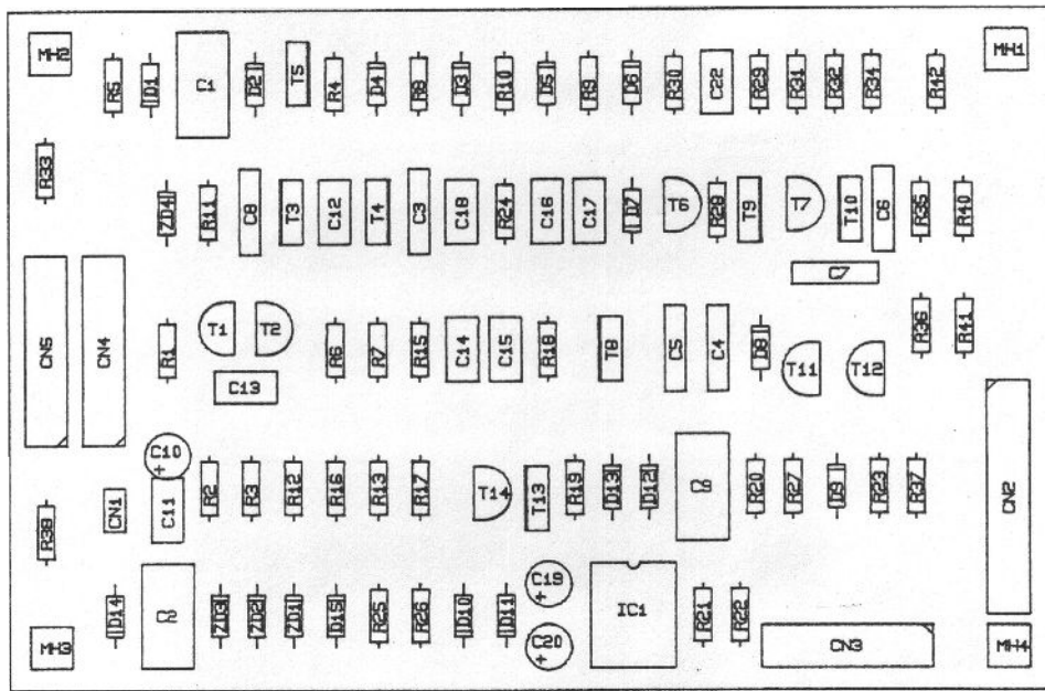
PAGE 22 preamp board
