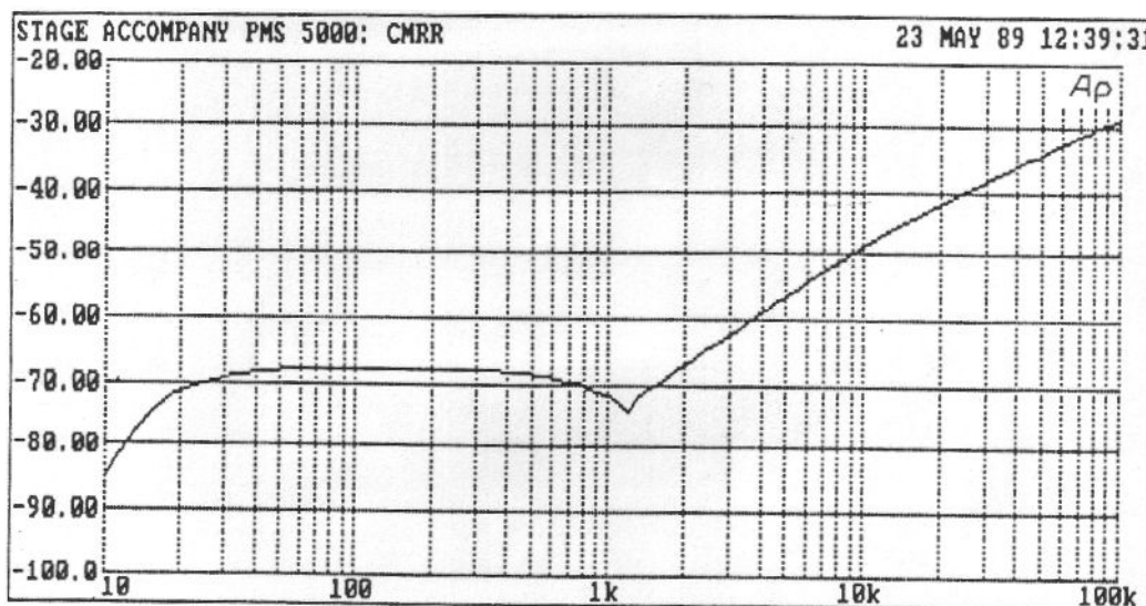
Fig 12 Typical CMR versus frequency
