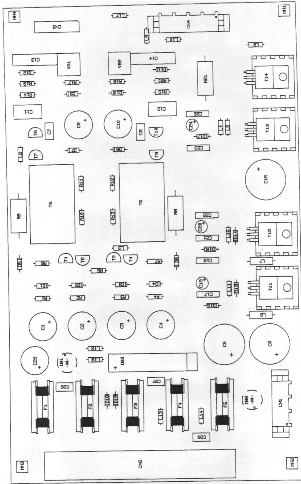
PAGE 26 regulated power supply board
