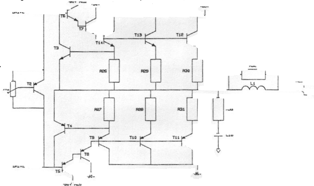
Fig 7 power amplifier
