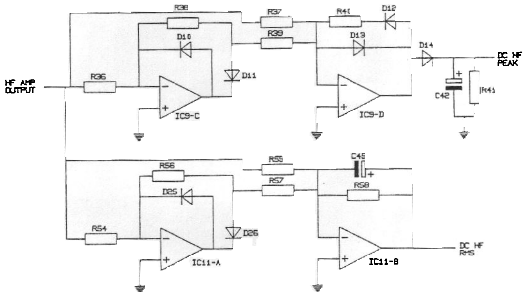
Fig 5 electronic rectifiers
