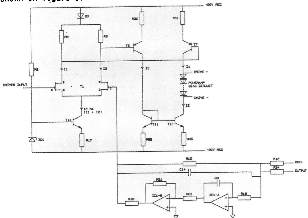
Fig 6 driver circuit
