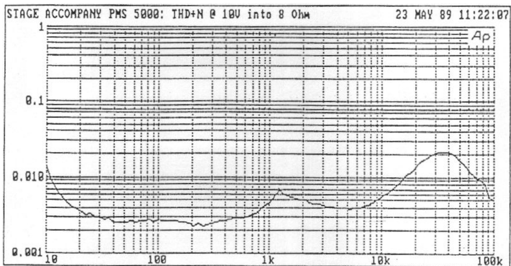
Fig 10 Typical harmonic distortion at 10 V / 8 \Omega
