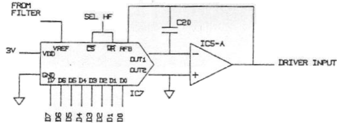
Fig 4 Digital attenuator
