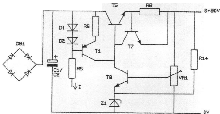
Fig 8 high voltage regulator
