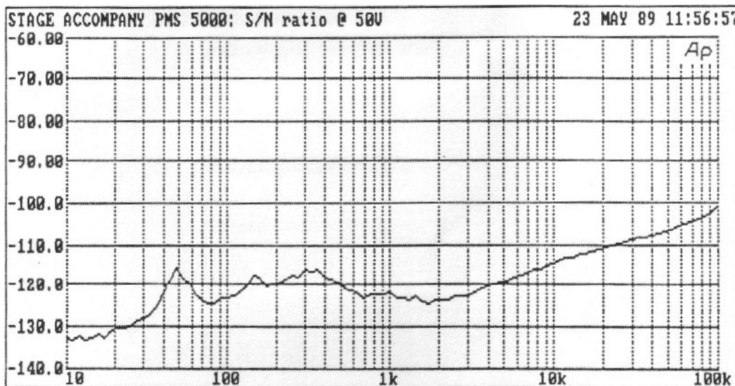
Fig 11 Output noise versus frequency, @ 0 dBm
