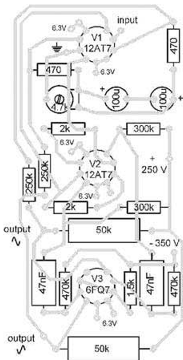
P.C.B. for STAX O.T.L. Amplifier (one channel) copper side view. Tubes sockets are soldered on this side.
