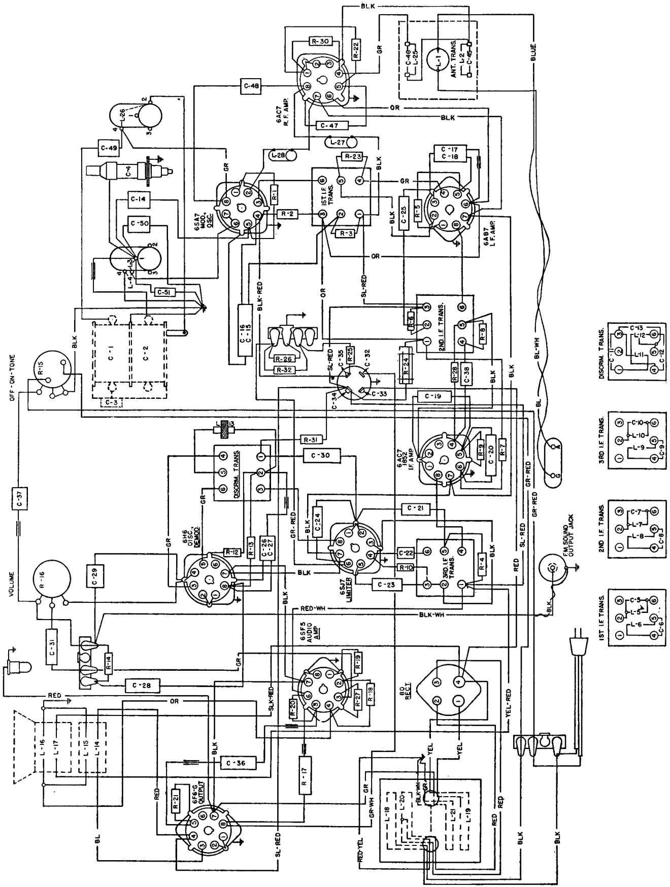
Wiring Diagram
