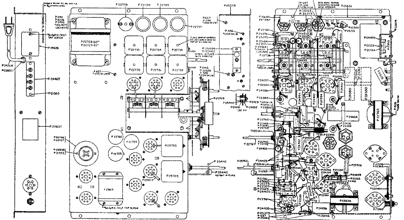
Fig. 3. Chassis Assembly.
