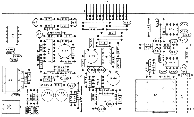
AUDIO PCB 1.726.820/821
