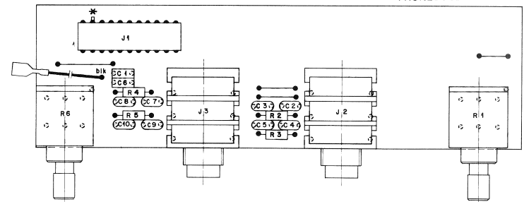
PHONES PCB 1.726.860
