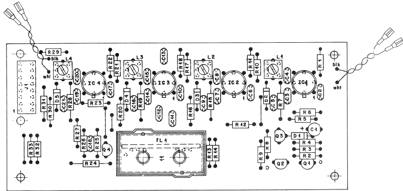
IF-AMPLIFIER PCB 1.726.740
