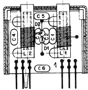
IF-DISCRIMINATOR PCB 1.726.741
