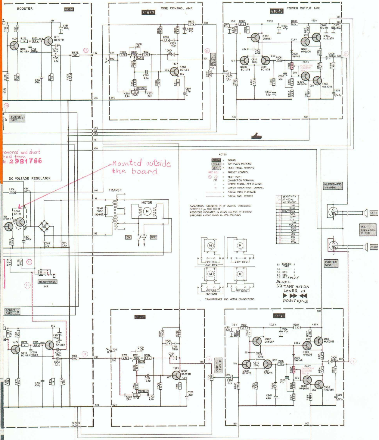
The Circuit Diagram of the 3400X tape recorder reel to reel machine.
