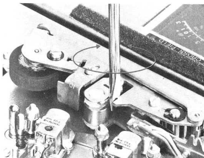
Fig. 2.16. Azimuth adjustment of inertia idling roller.
