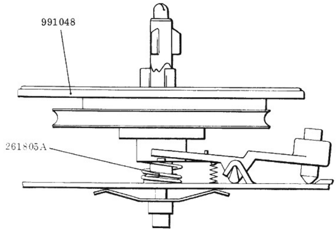
Fig. 2.5. Supply turntable, operating lever in reverse winding.
