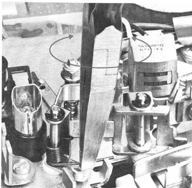
Fig. 2.14. Adjustment of pressure pad tension.
