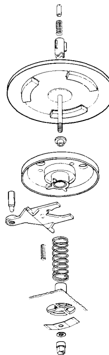
Fig. 3.5 The supply turntable
