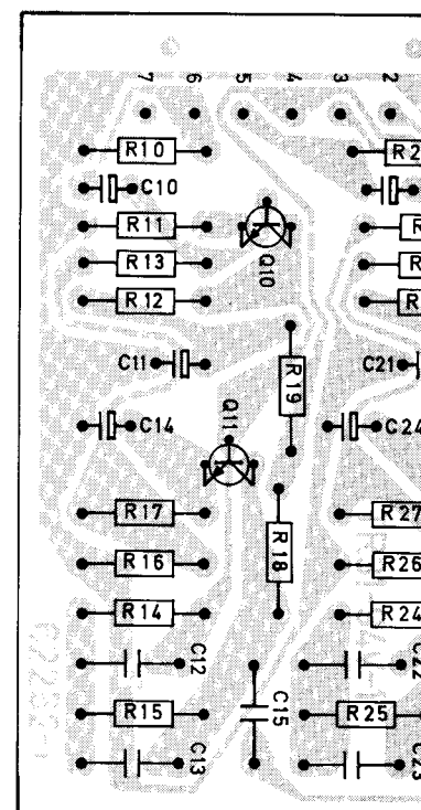
PHONO AMP
