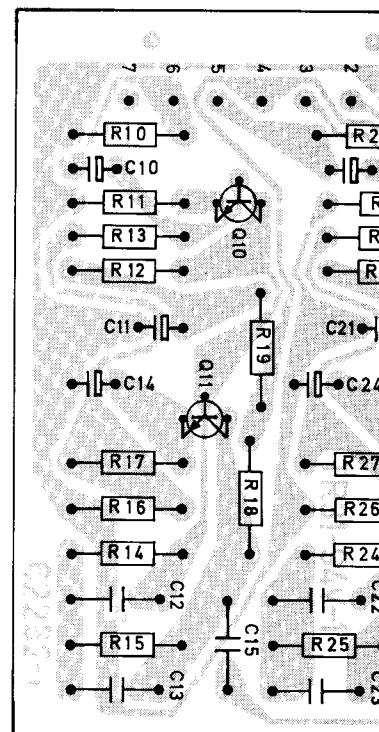
PHONO AMP
