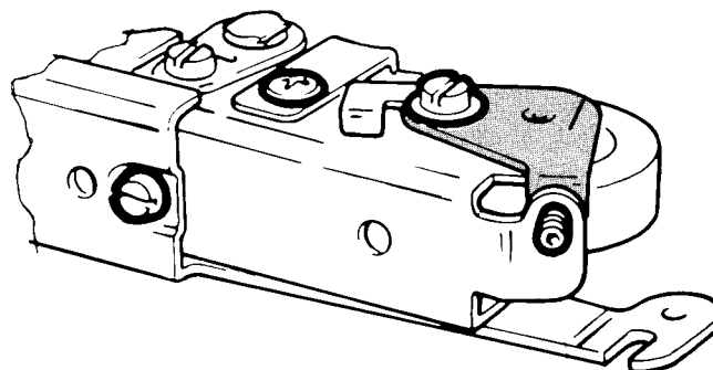
Fig. 4.4. Adjusting the pinch roller.
