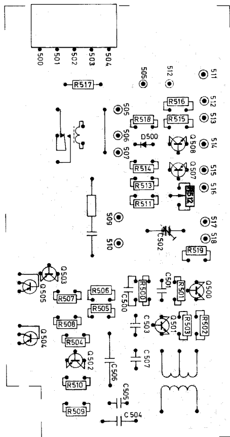
OSCILLATOR
