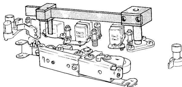
Fig. 4.2. Adjusting with the tape path gauge.
