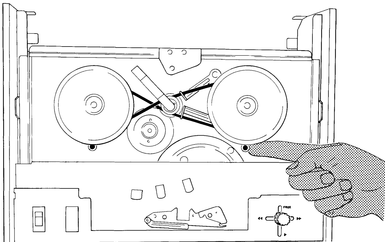
Fig. 3.6 Checking the play on the clutch levers
