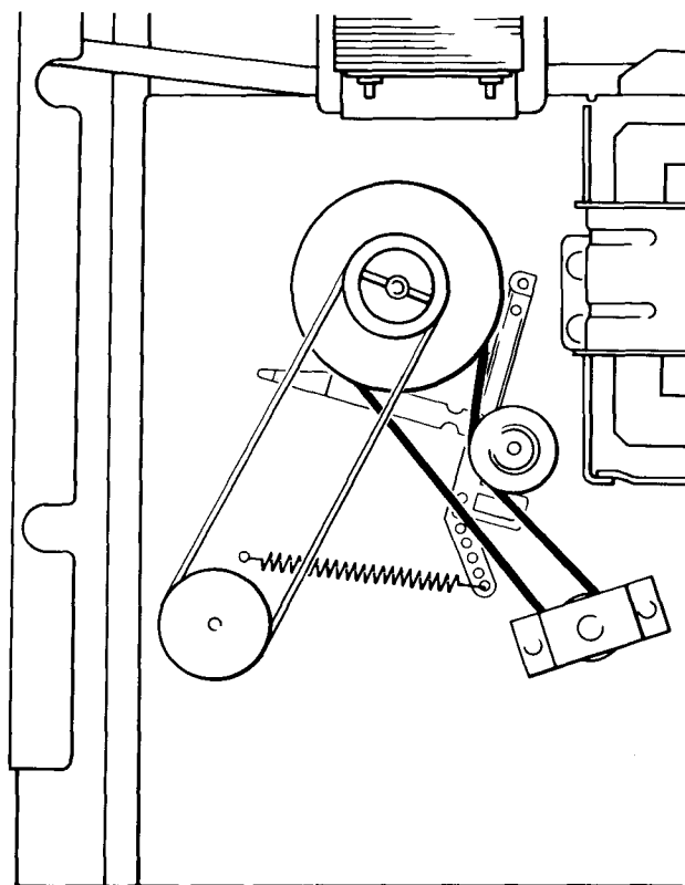
Fig. 3.3 Adjusting the take-up force.
