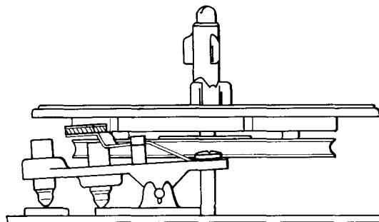
Fig.3.8. Adjusting the brakes on the right turntable
