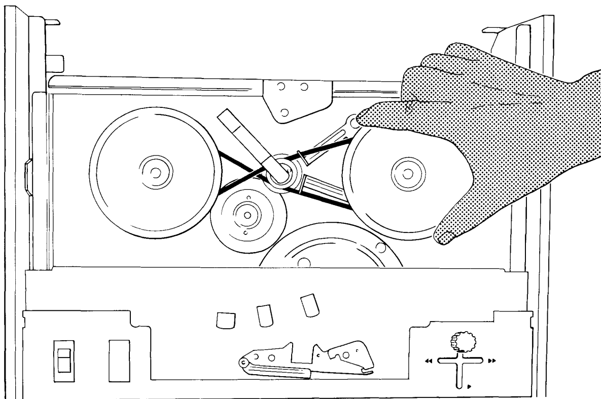
Fig. 3.4 Checking the play on the turntables
