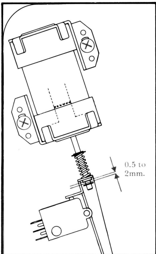
Fig. 3.3 The pinch roller solenoid
