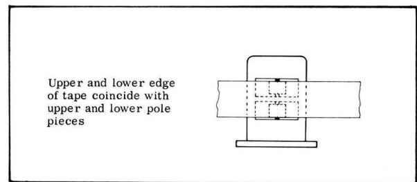
Fig. 6.6 Two-track playback head
