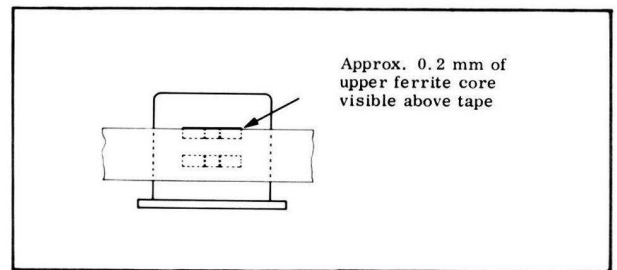
Fig. 6.4 Four-track erase head.
