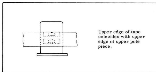
Fig. 6.2 Four-track record head.
