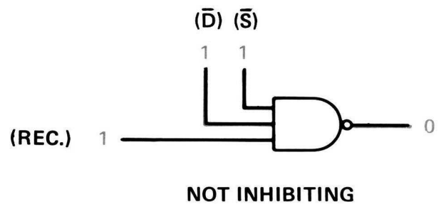
Fig. 1.10 Inhibitor-circuit
