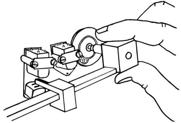
Fig. 5.1 Adjusting the parallelism with the head tool.
