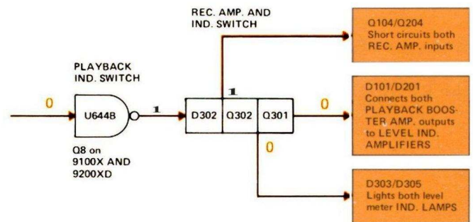
Fig. 2.6 Meter-switch operation during playback
