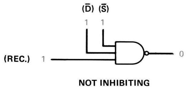
Fig. 1.10 Inhibitor-circuit
