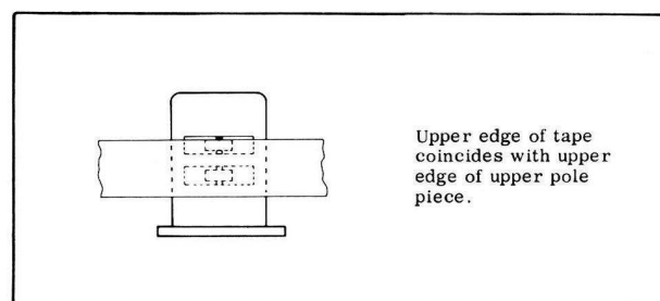
Fig. 6.2 Four-track record head.
