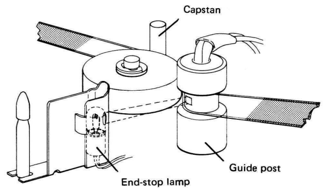
Fig. 11.1 The photo-electric end-stop
