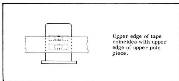
Fig. 6.5 Four-track playback head
