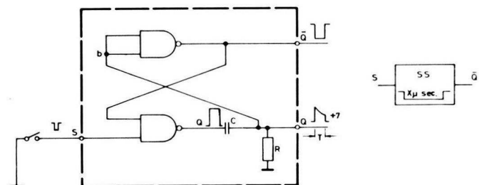
Fig. 1.6 Monostable circuit and symbol
