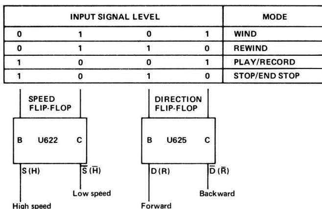
Fig. 2.4 Speed flip-flop and direction flip-flop
