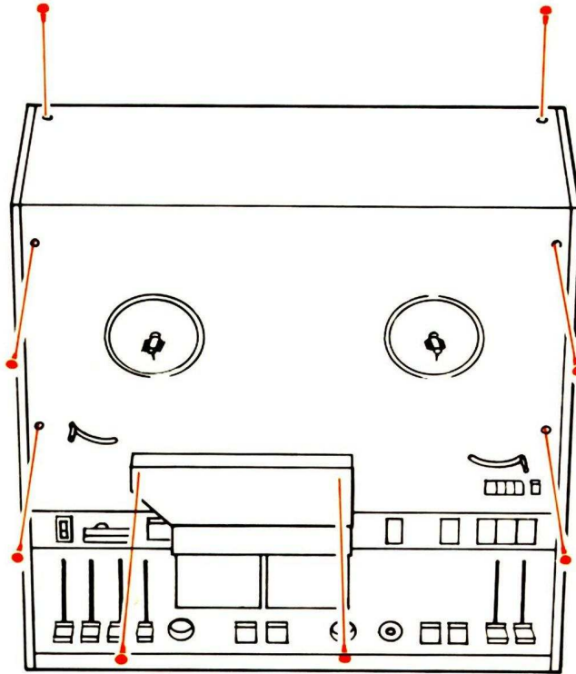
Fig. 1.1 The screws for the front plate.
