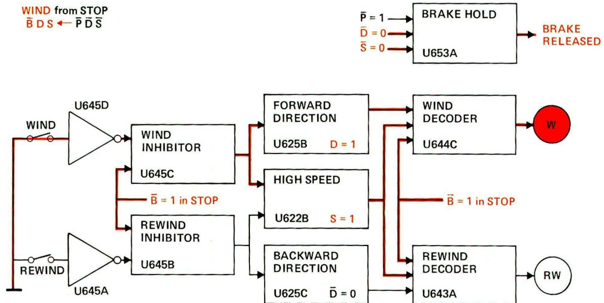
Fig. 3.8 WIND from STOP
