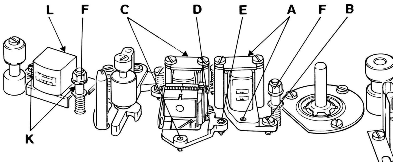
Fig. 6.1 The head adjustment screws
