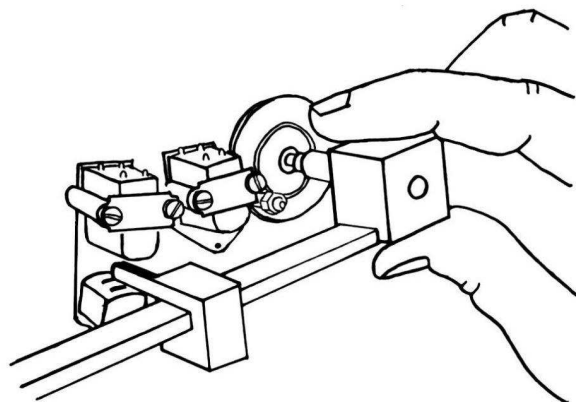
Fig. 5.1 Adjusting the parallelism with the head tool.
