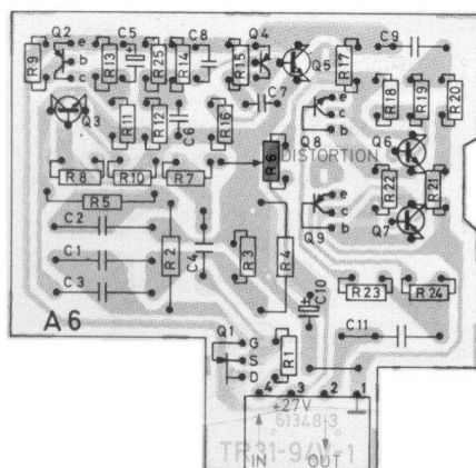
A6 OSCILLATOR BOARD MODEL 9100X AND 9200XD
