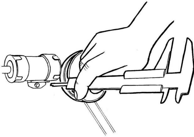
Fig. 3.4 Checking the height of the turntable
