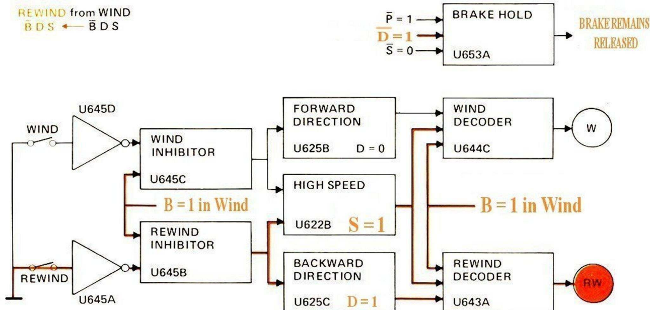
Fig. 3.9 REWIND from WIND
