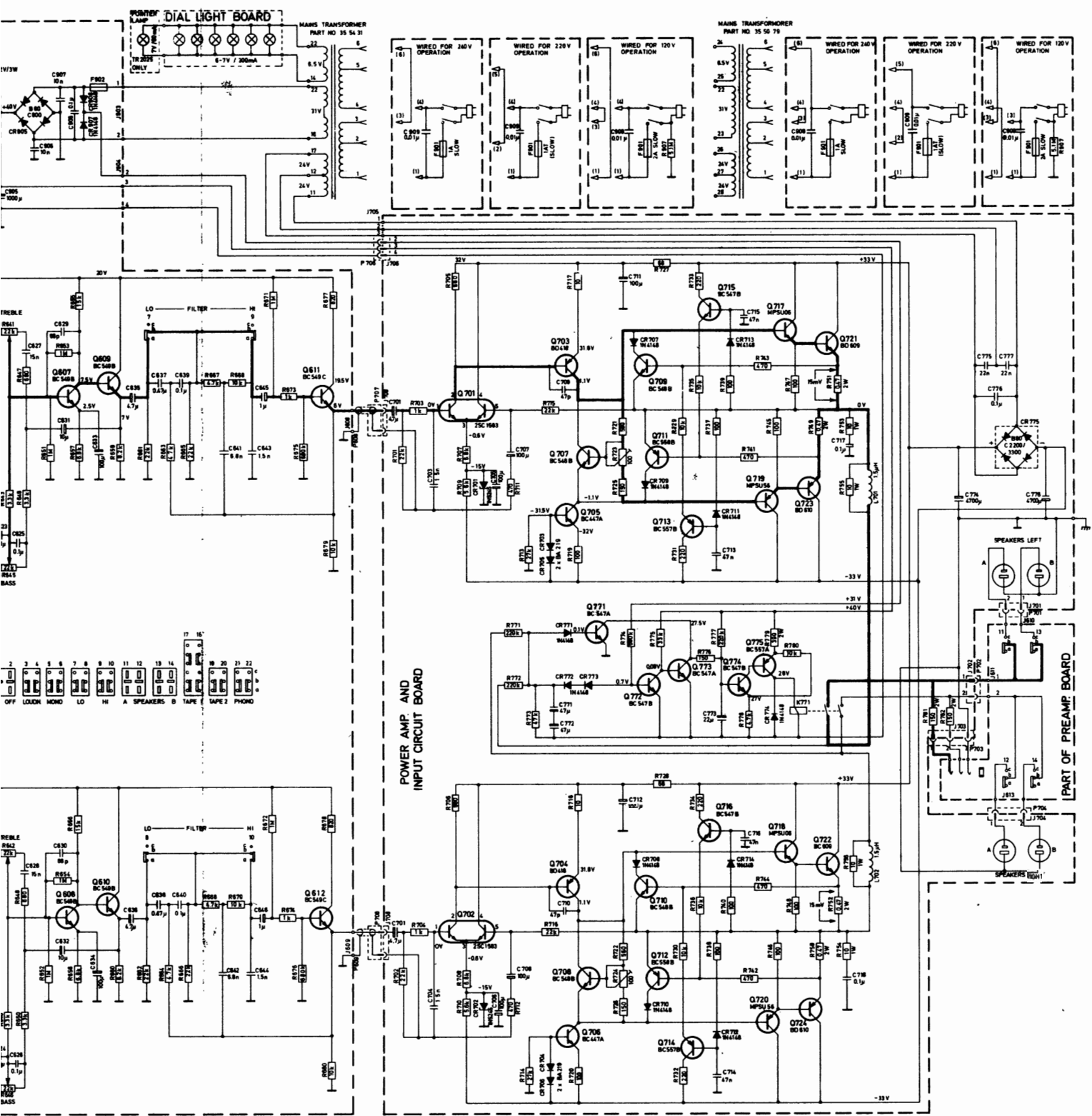
AUDIO-FREQ. SECTION NO. 44233.
