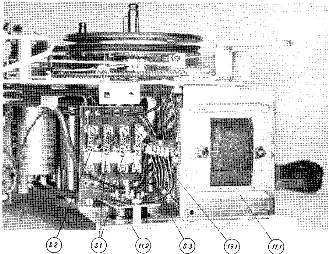
Fig. 31. Fuse Board
