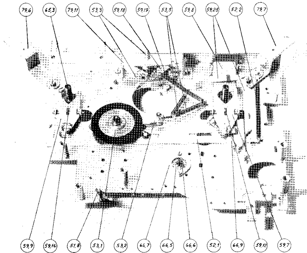
Fig. 29. Lower Mounting Plate, Upper Mounting Plate Removed.
