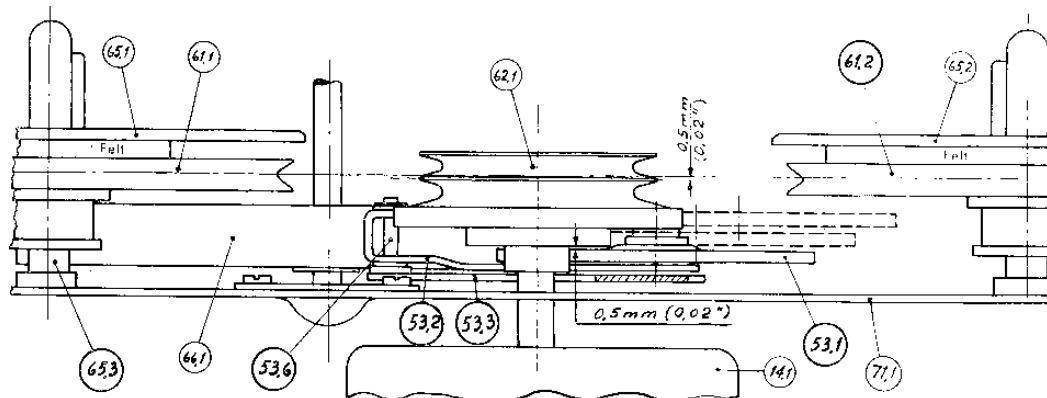
Fig. 14. Driving Mechanism
