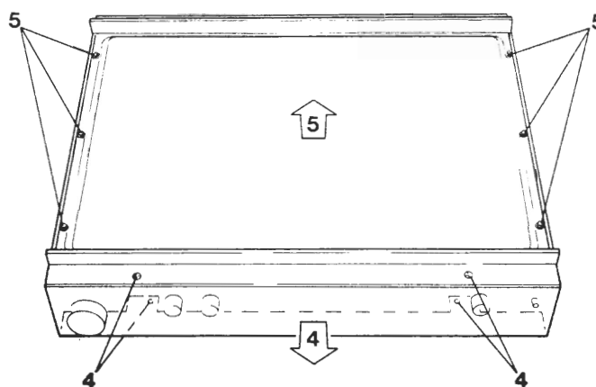
Dismantling the front and bottom covers
