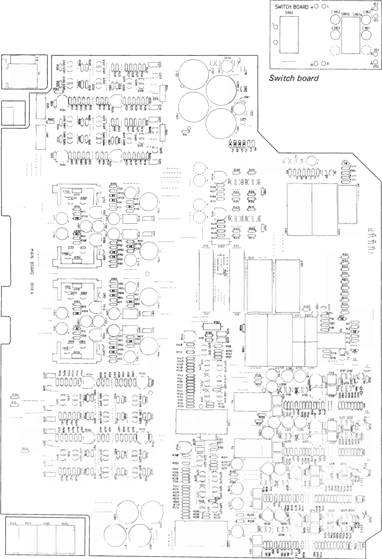
Main board
