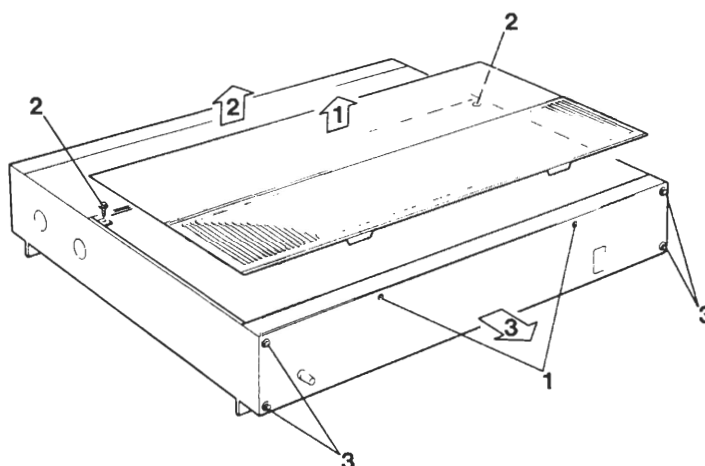
Dismantling the rear and top covers
