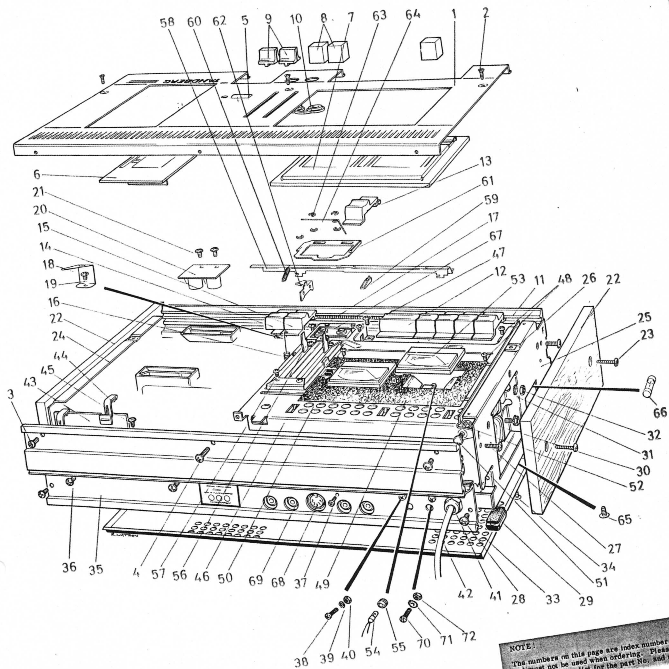
FIG. 1. CHASSIS ASSEMBLY
