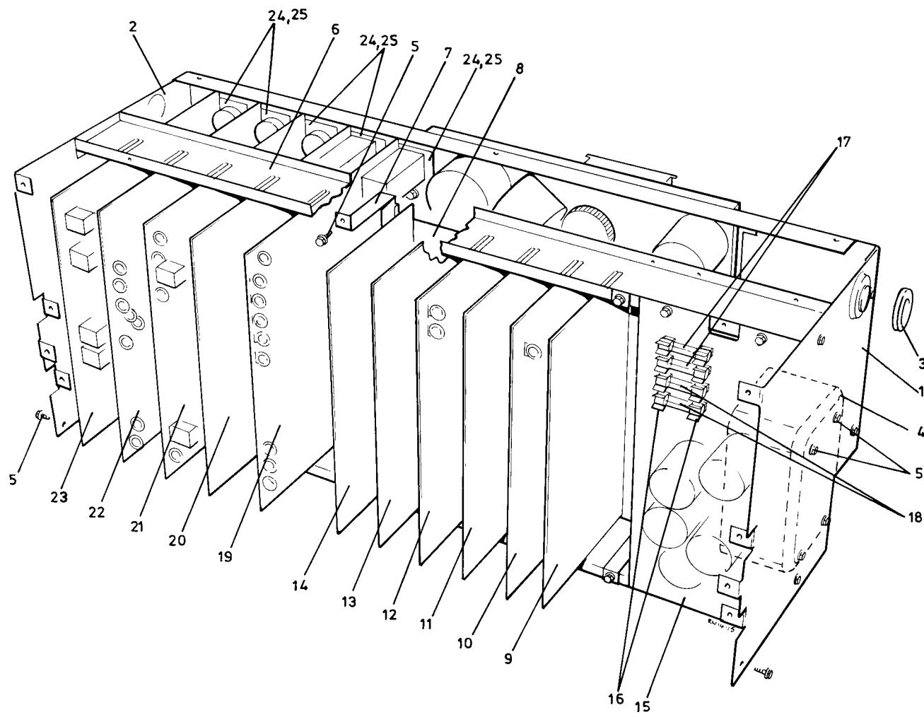
Chassis assembly - top rear view
