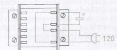
Powertransformer, part No. 352622, UI 48/26 TD2600
