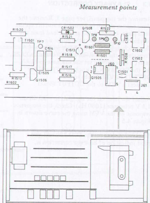
Fig. 4.6 Measurement points on the oscillator board
