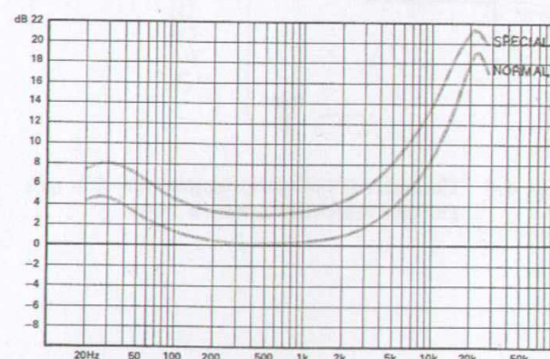
Fig. 4.7 Record correction
