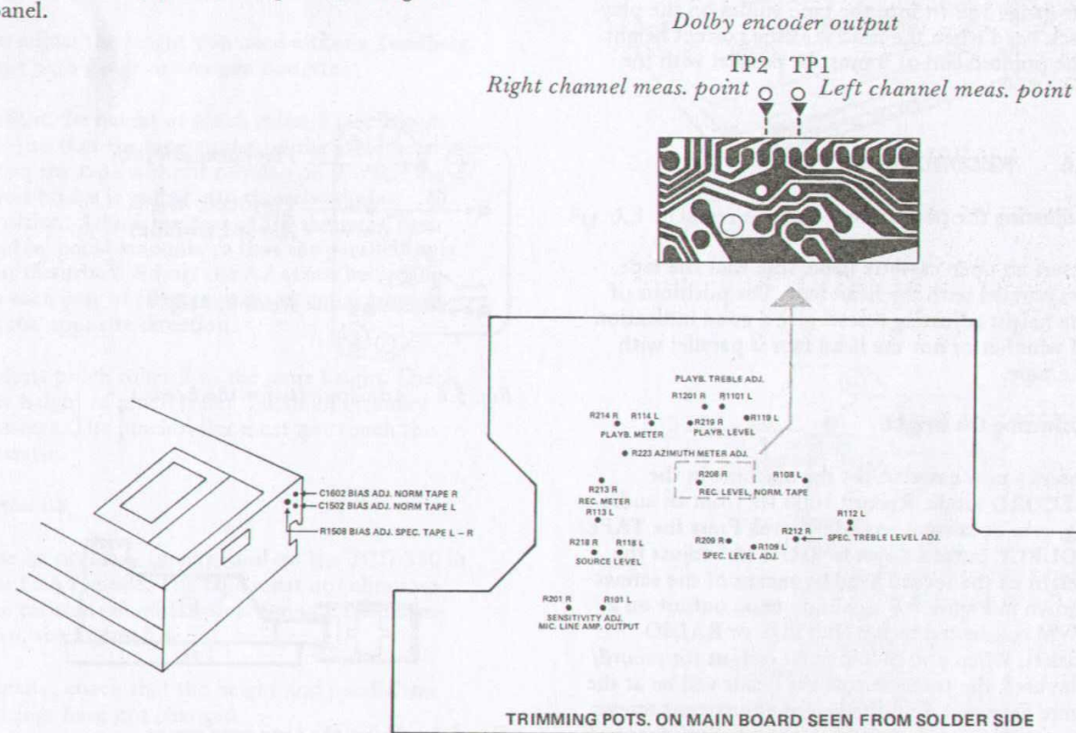
Fig. 6.1 Trimming pots. and Dolby encoders measurement points
