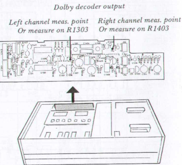
Fig. 6.2 Dolby decoder measurement points
