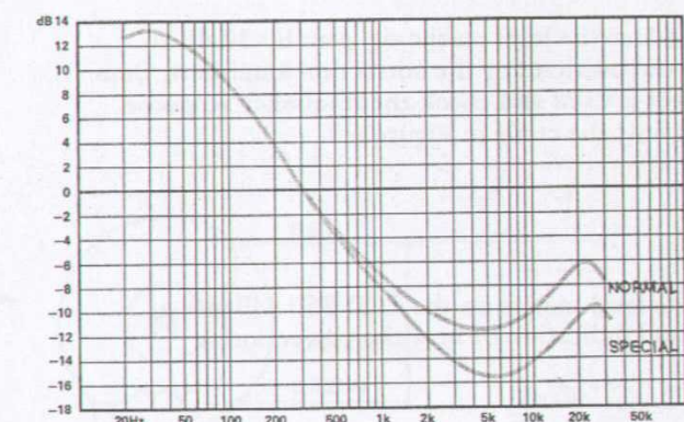
Fig. 4.5 Playback correction
