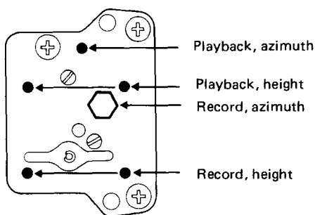
Figure 3 Adjustments for the heads
