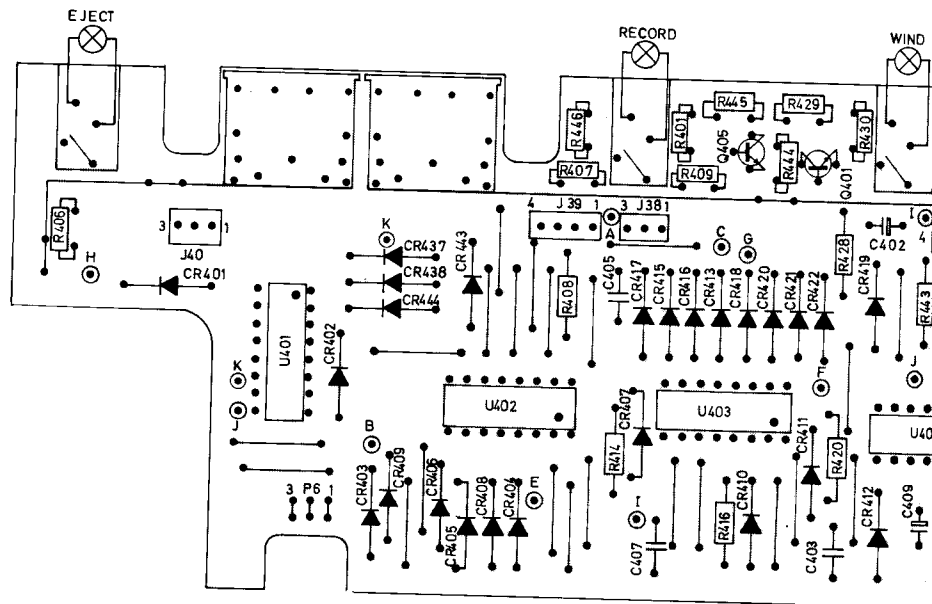
A2 LOGIC BOARD
