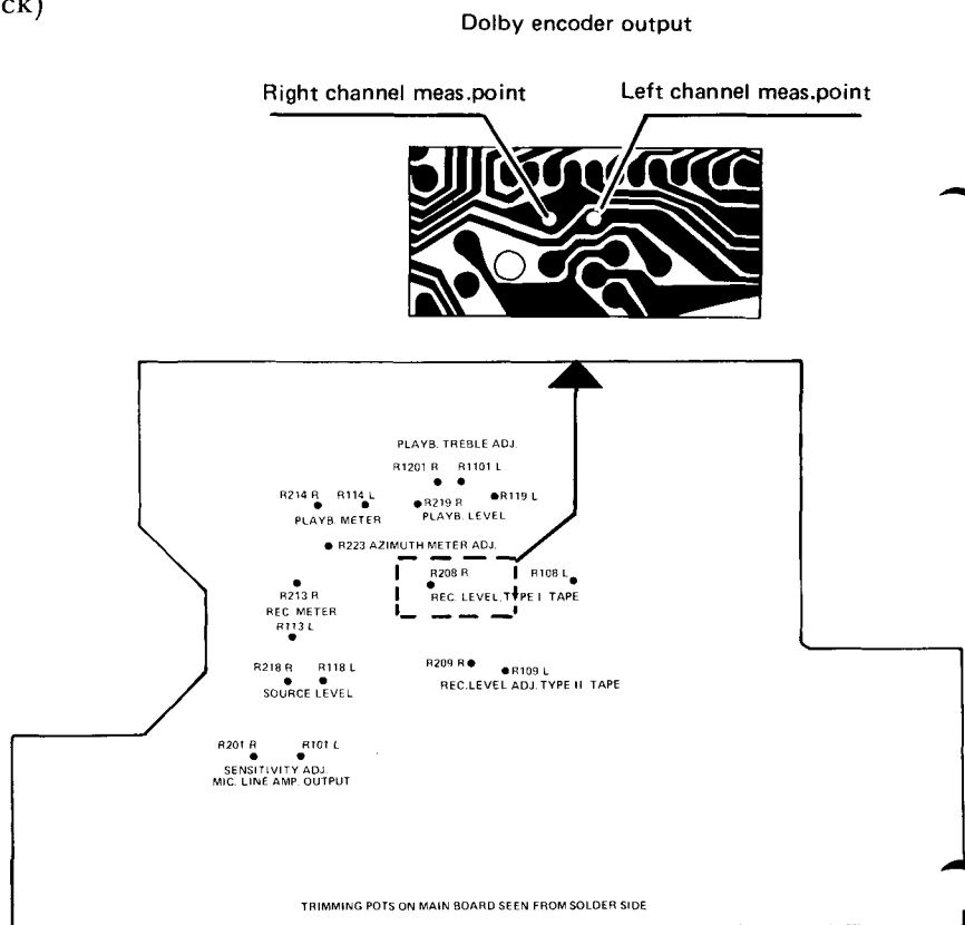
Figure 1 Trimming pots. and Dolby encoder measurement points
