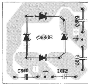
Figure 11, Rectifier board, solder side
