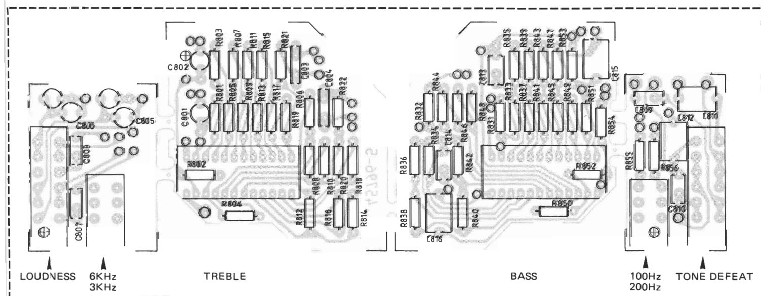
Figure 12, Tone control boards, component side
