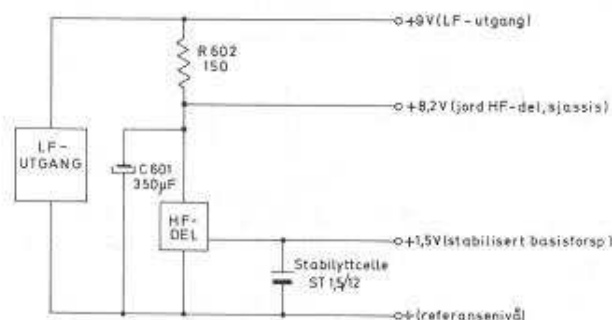
Fig. 2. Likespenningnivåer.
