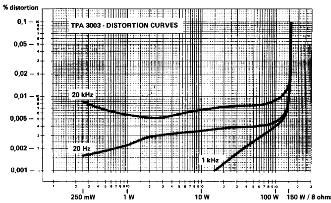
Total harmonic distortion versus output power
