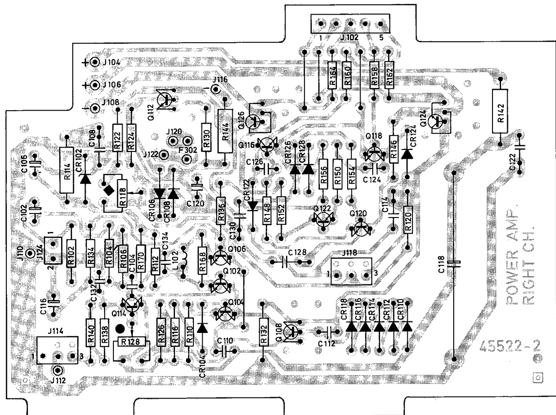
Power amplifier board, right channel
