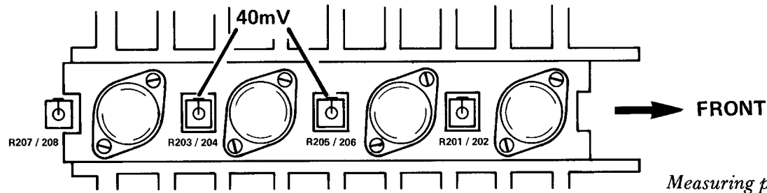
Measuring point, quiescent current.
