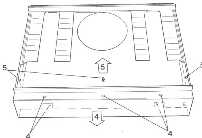
Dismantling the front and bottom covers.
