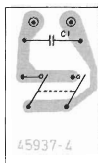
Power switch board, solder side
