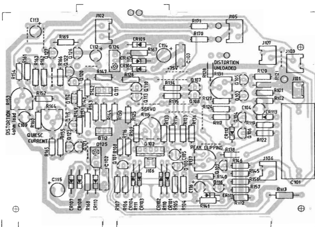
Power amplifier board, component side
