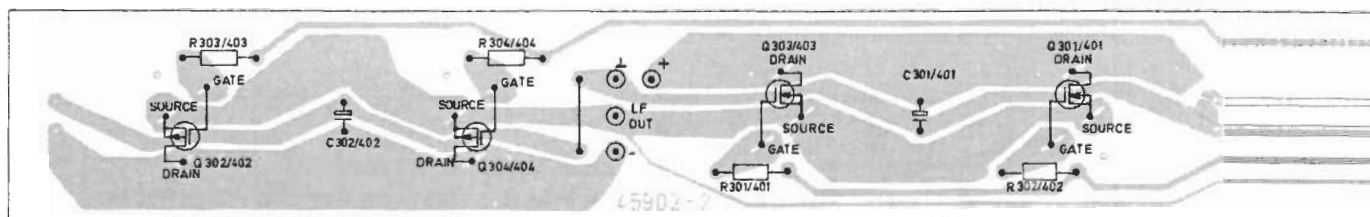
Output power amplifier board, solder side
