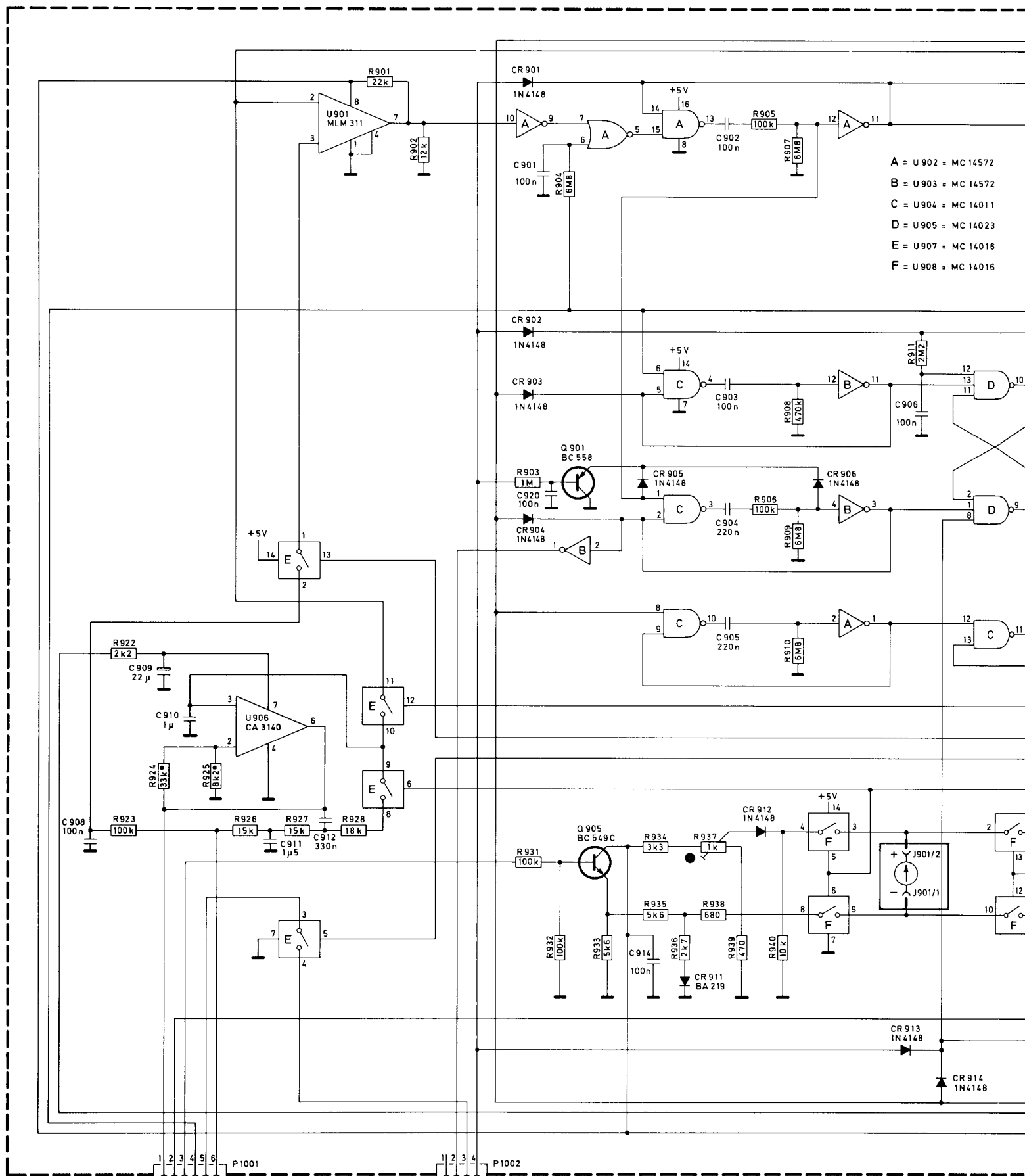
Figure 41 Tuning system 1
