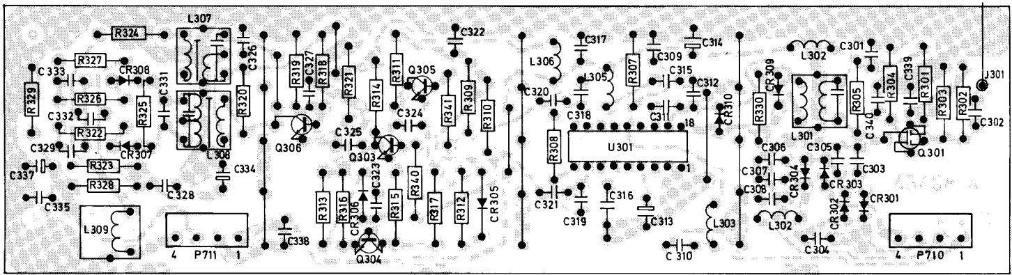
Figure 23 Limiter/detector board above serial No. 00700, foil side
