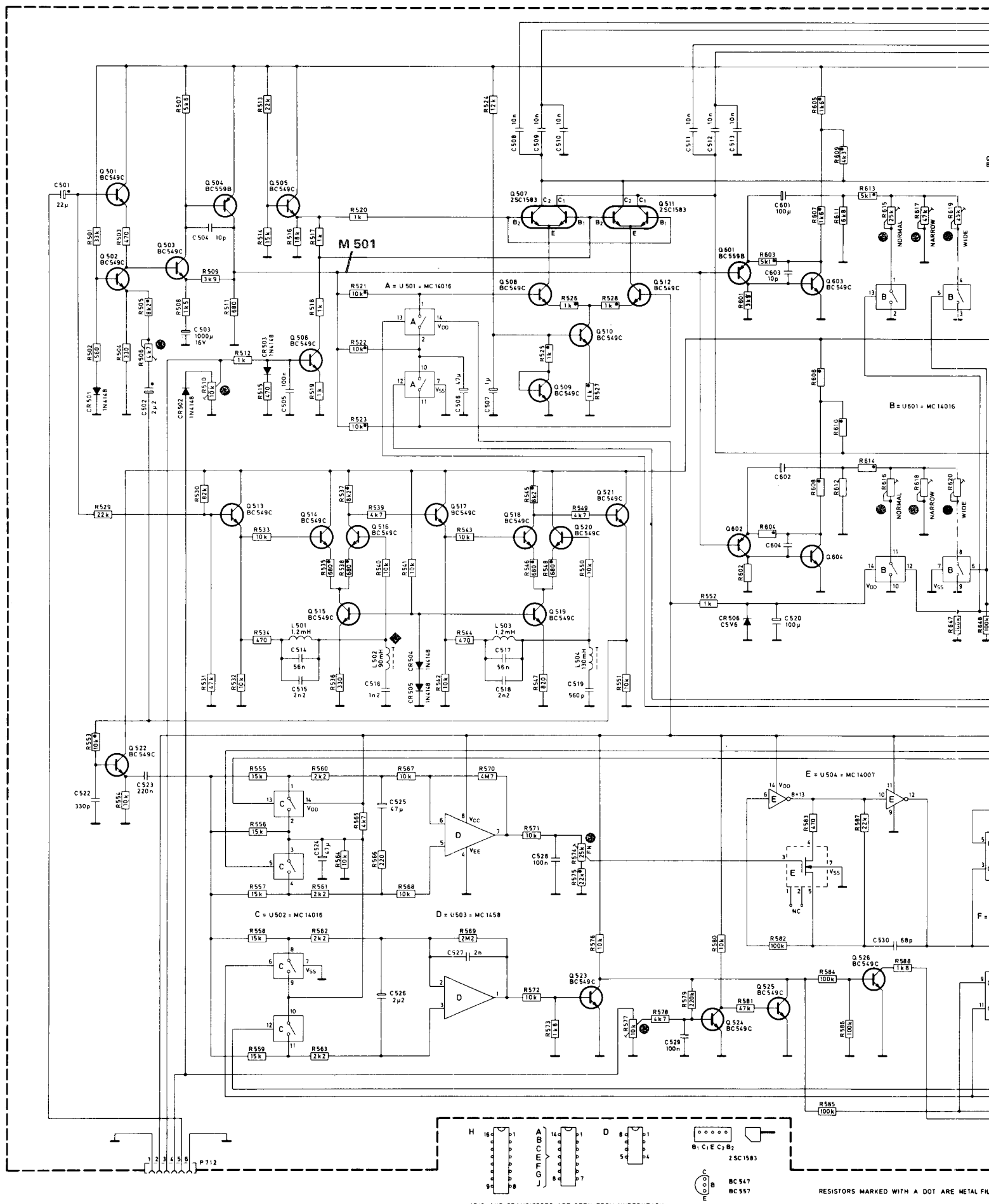
Figure 48 Stereo decoder
