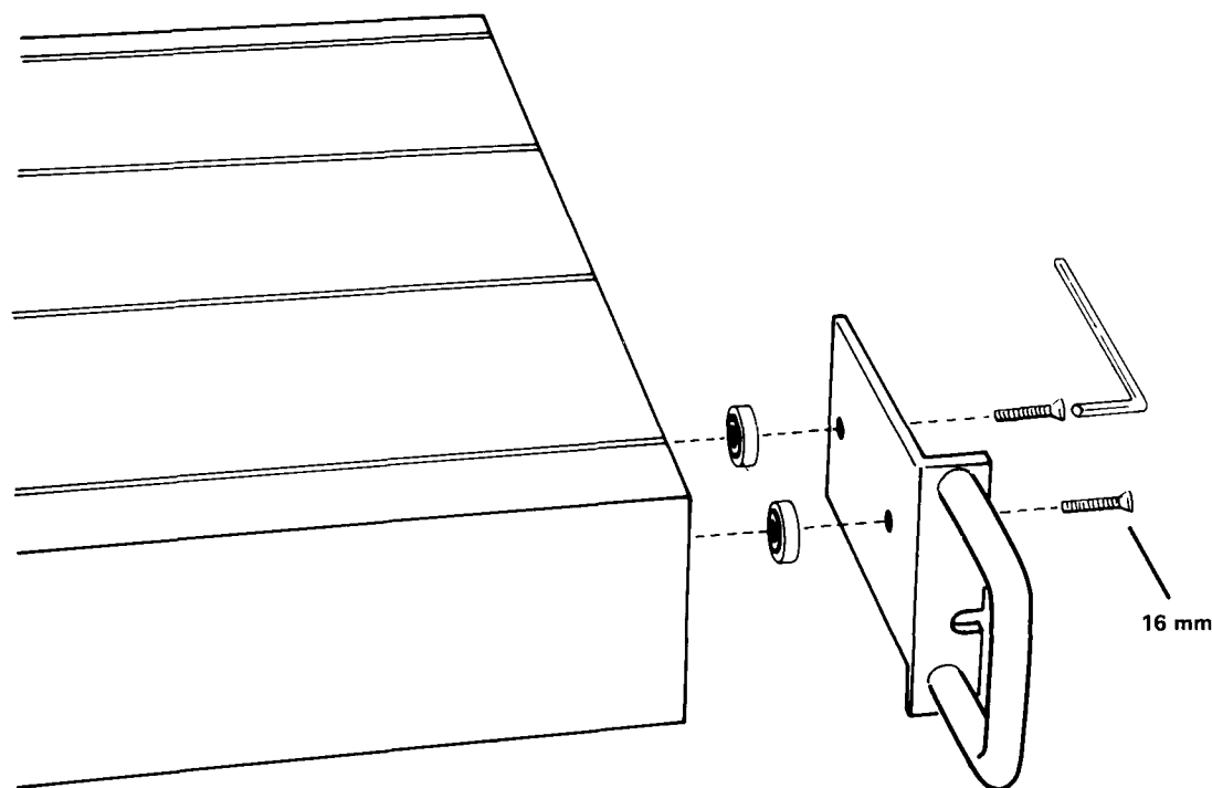
Figure 6 Mounting the 19"-rack mount kit (extra)
