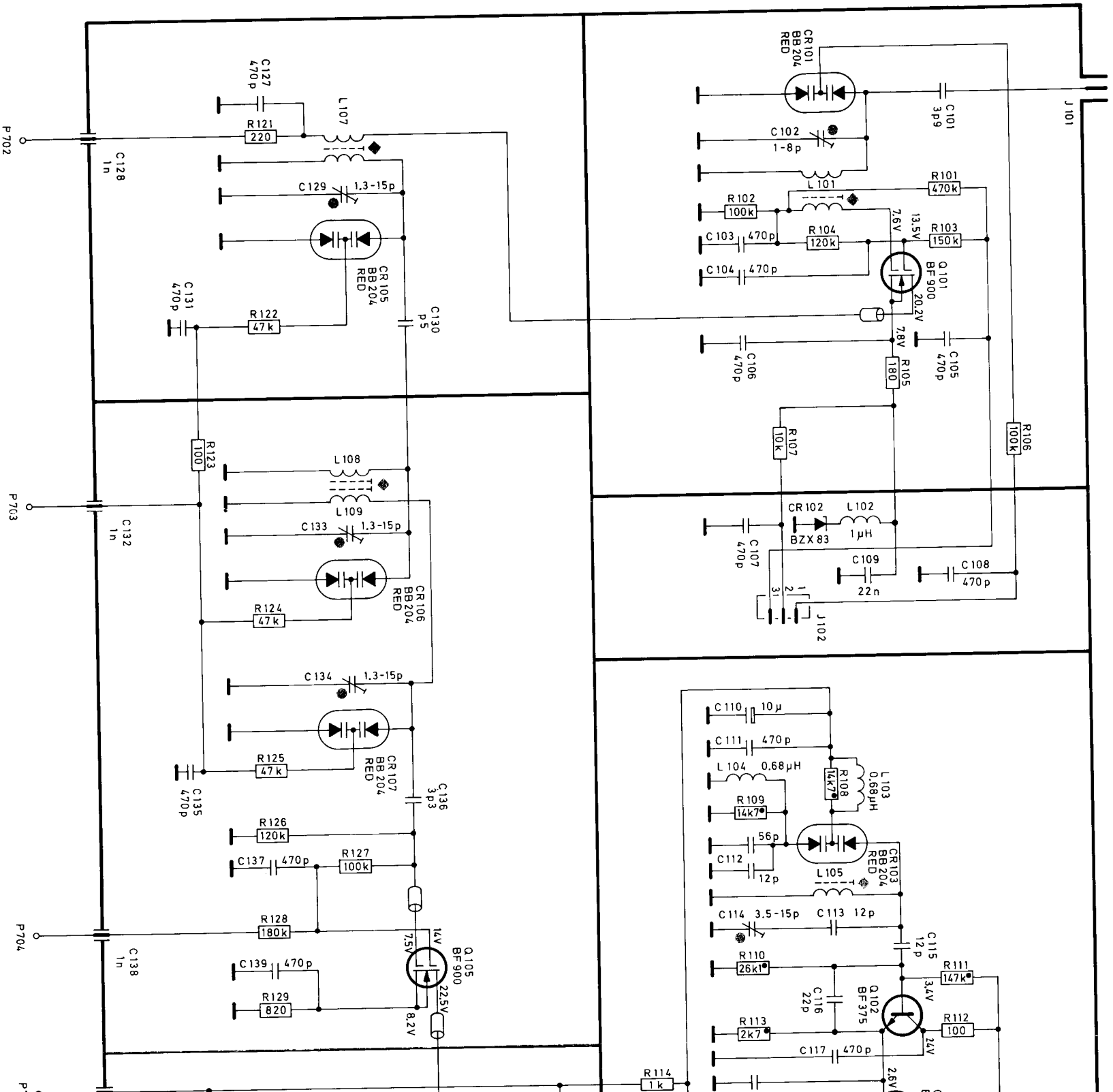
Figure 12 Front end
