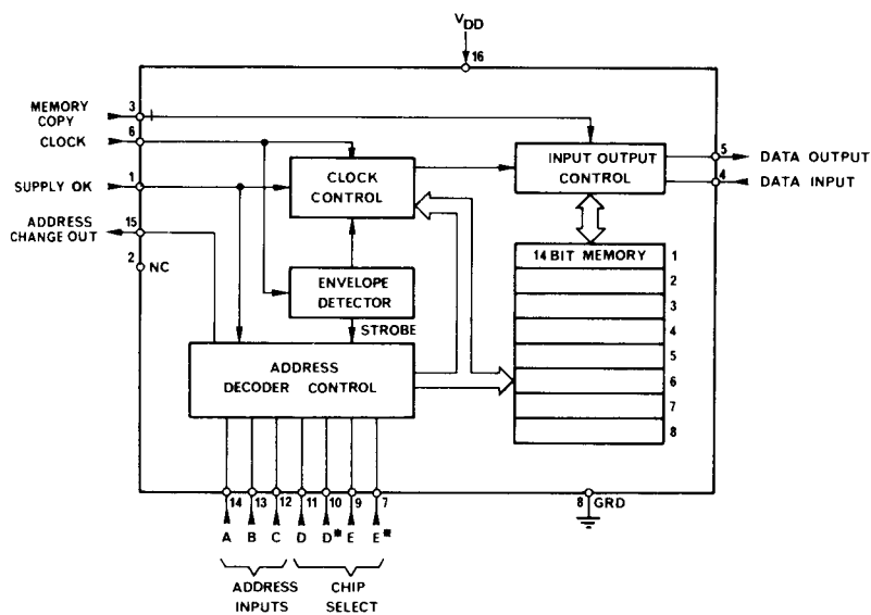
U1003 MC14426
