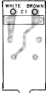
Figure 58 Power switch board, component side
