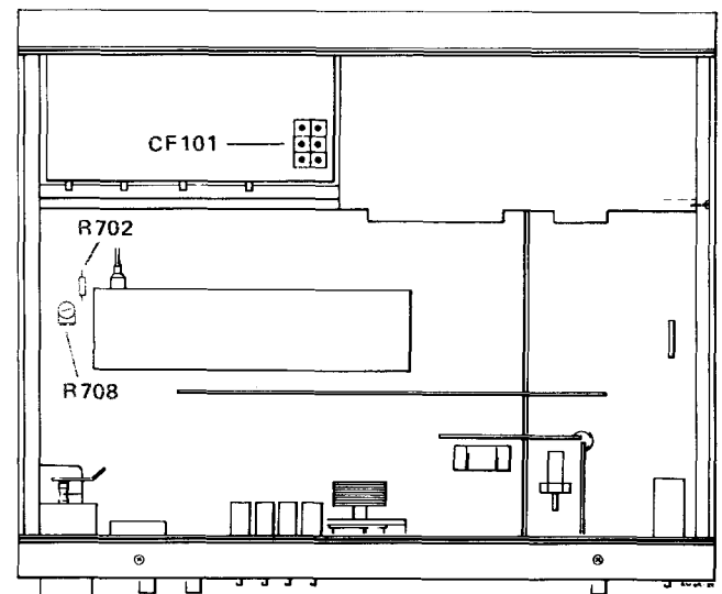
Figure 37 Test points
