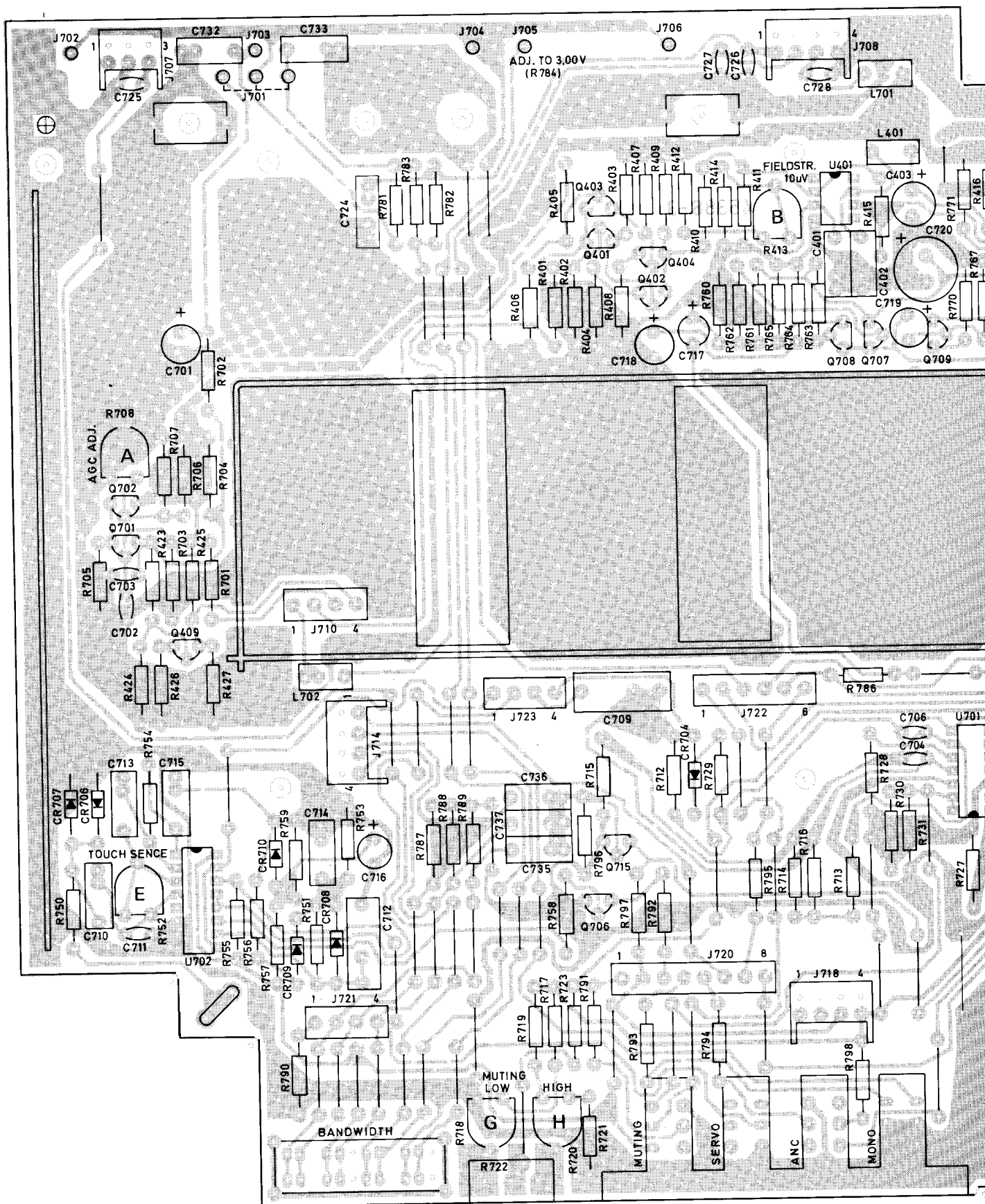
Figure 39 Main board, component side
