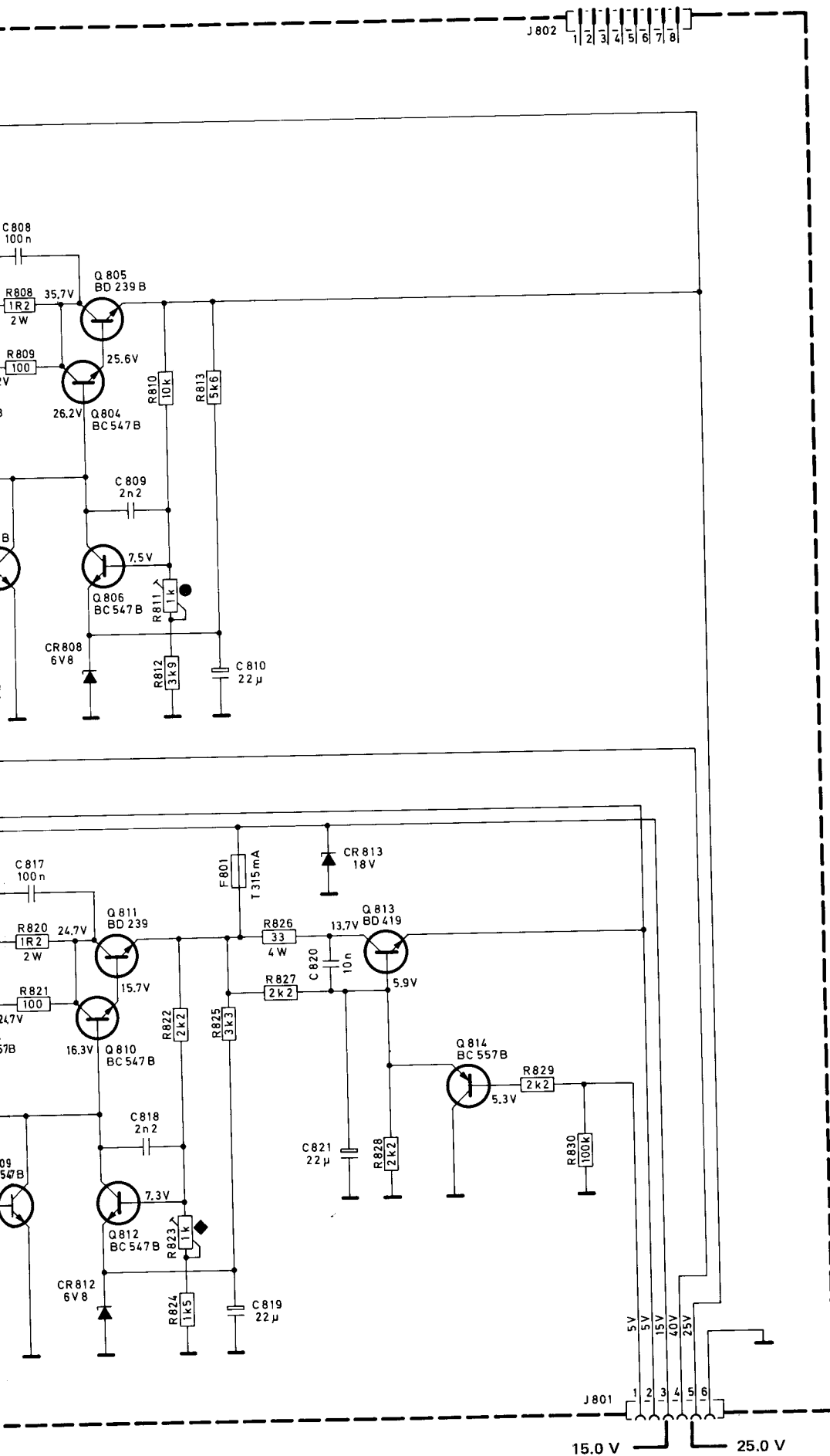
Figure 8 Power supply
