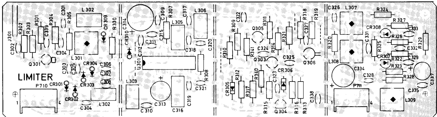
Figure 24 Limiter/detector board above serial No. 00700, component side
