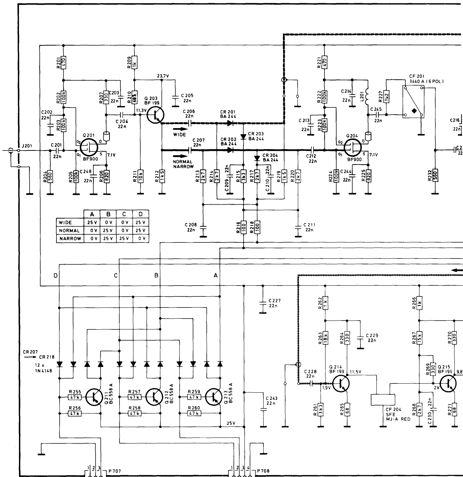
Figure 33 Selectivity circuit, above serial No. 00700
