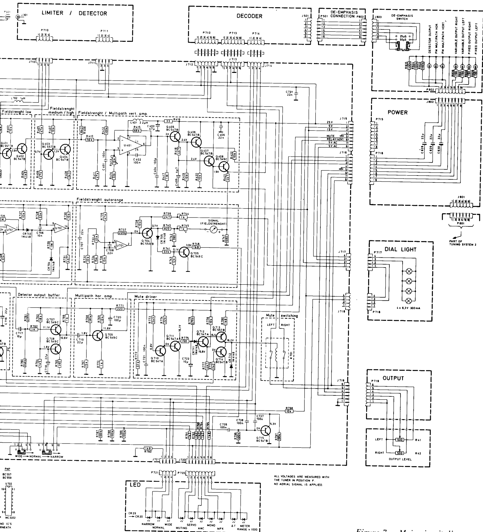
Figure 7 Main circuit diagram
