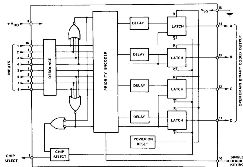
U1004 MC14430
