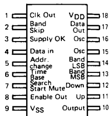
U1001 MC14429
