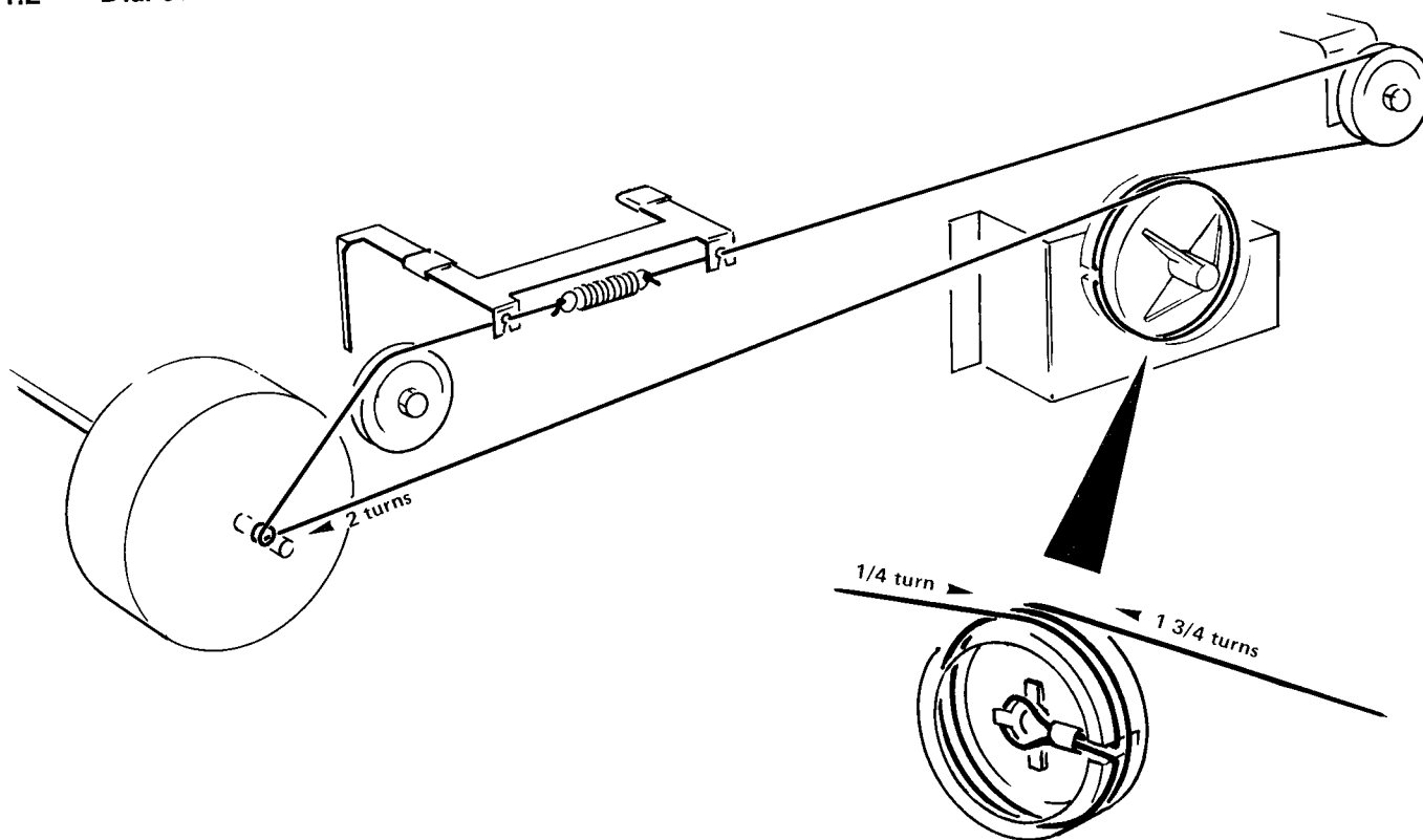
Figure 3 Dial cord drive
