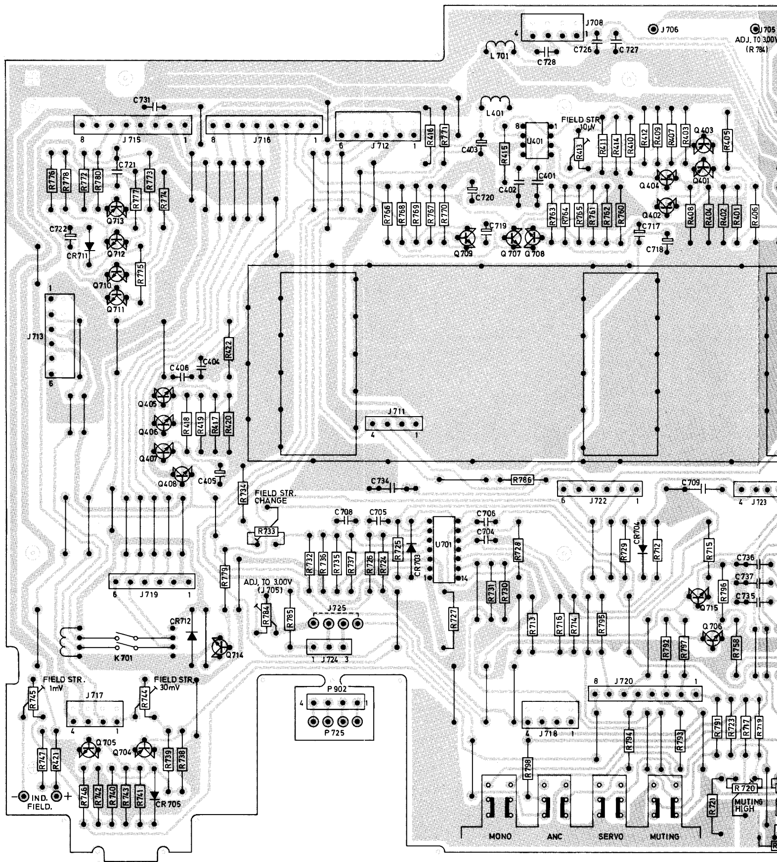
Figure 40 Main board, foil side
