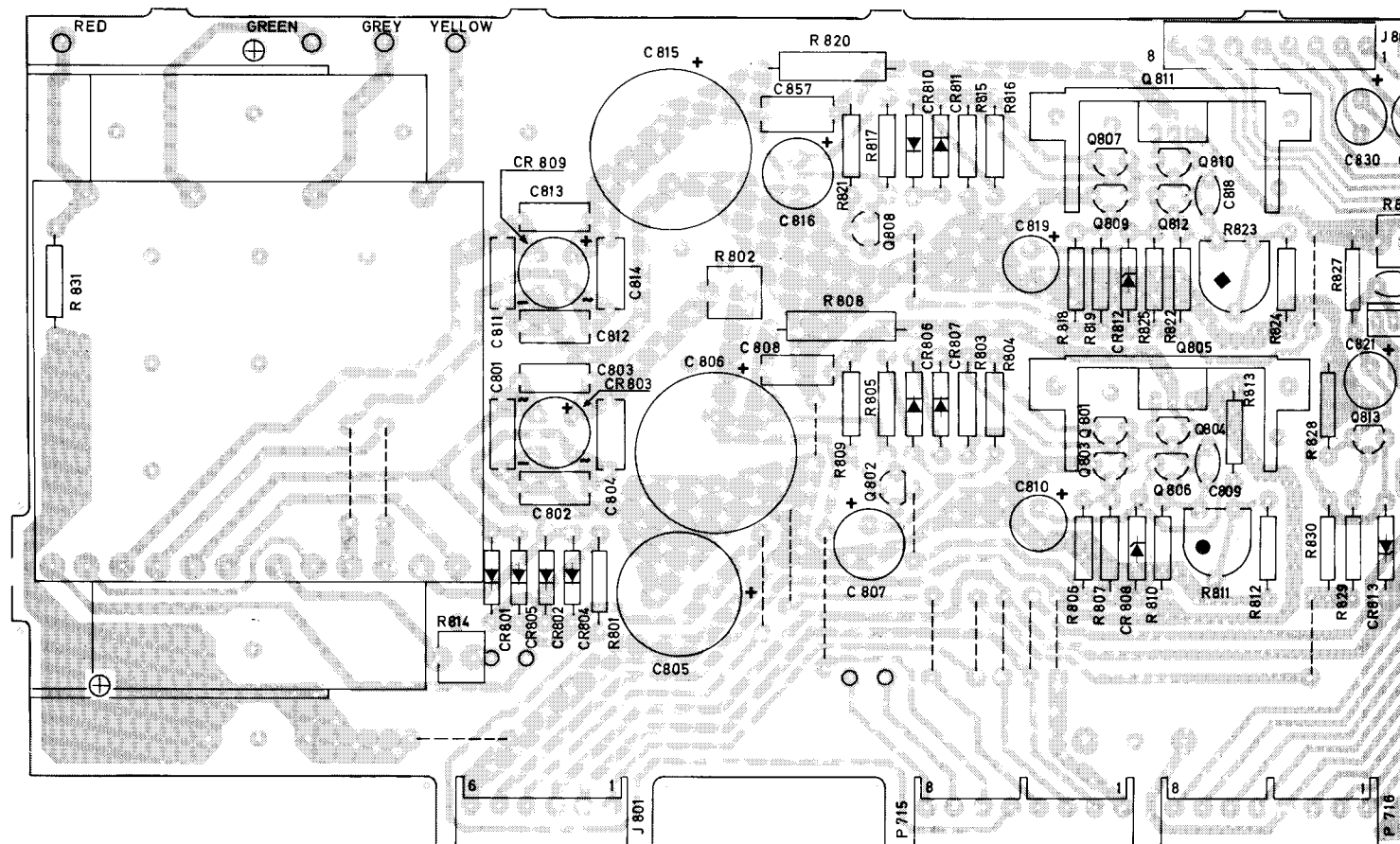
Figure 10 Power supply board, component side
