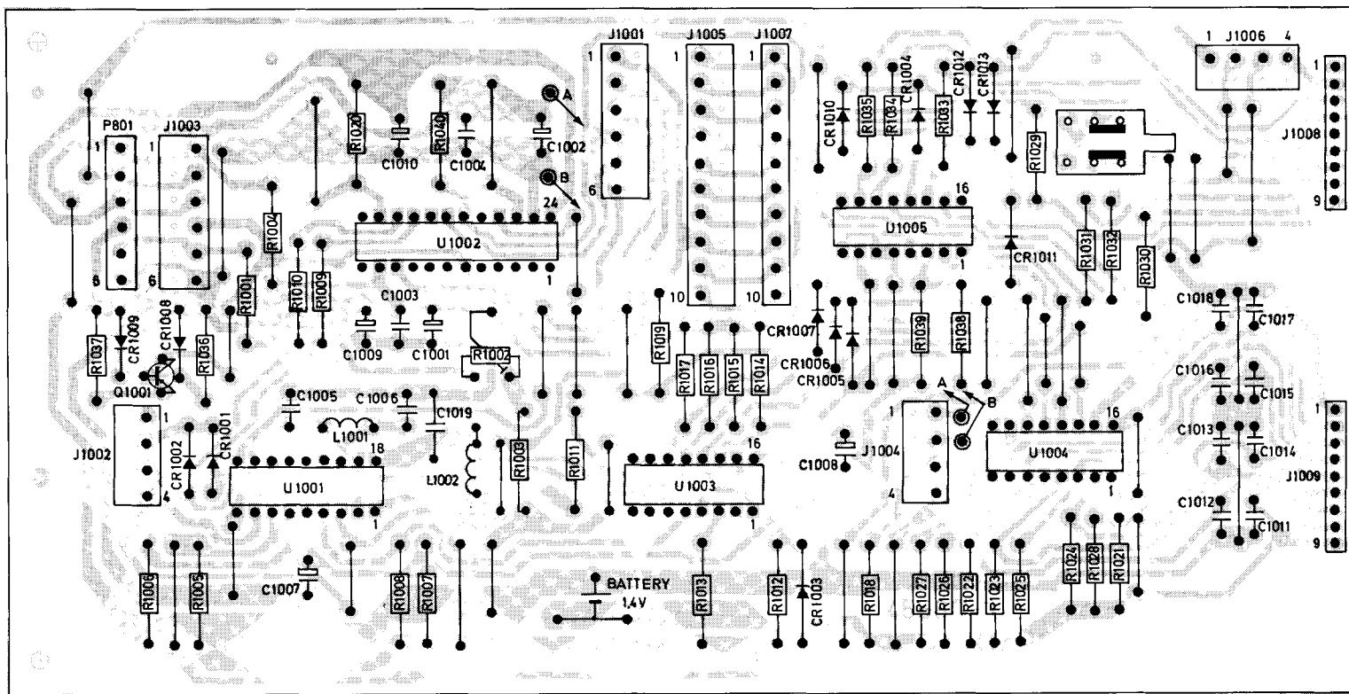
Figure 46 Tuning system 2 board, foil side
