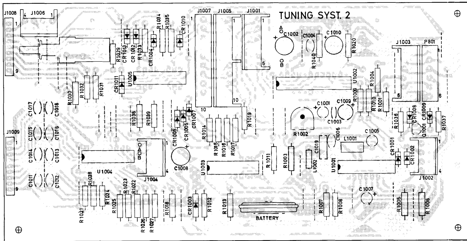
Figure 47 Tuning system 2 board, component side
