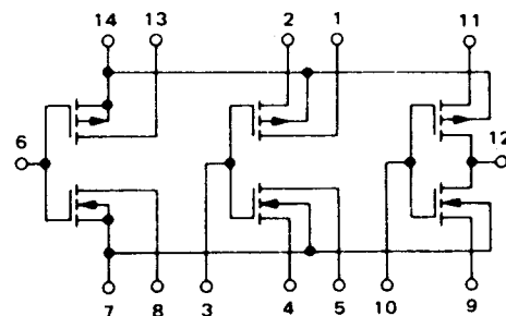
U504 MC14007
