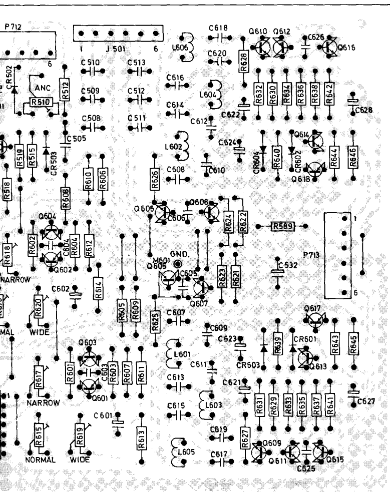
Figure 51 Stereo decoder board, foil side
