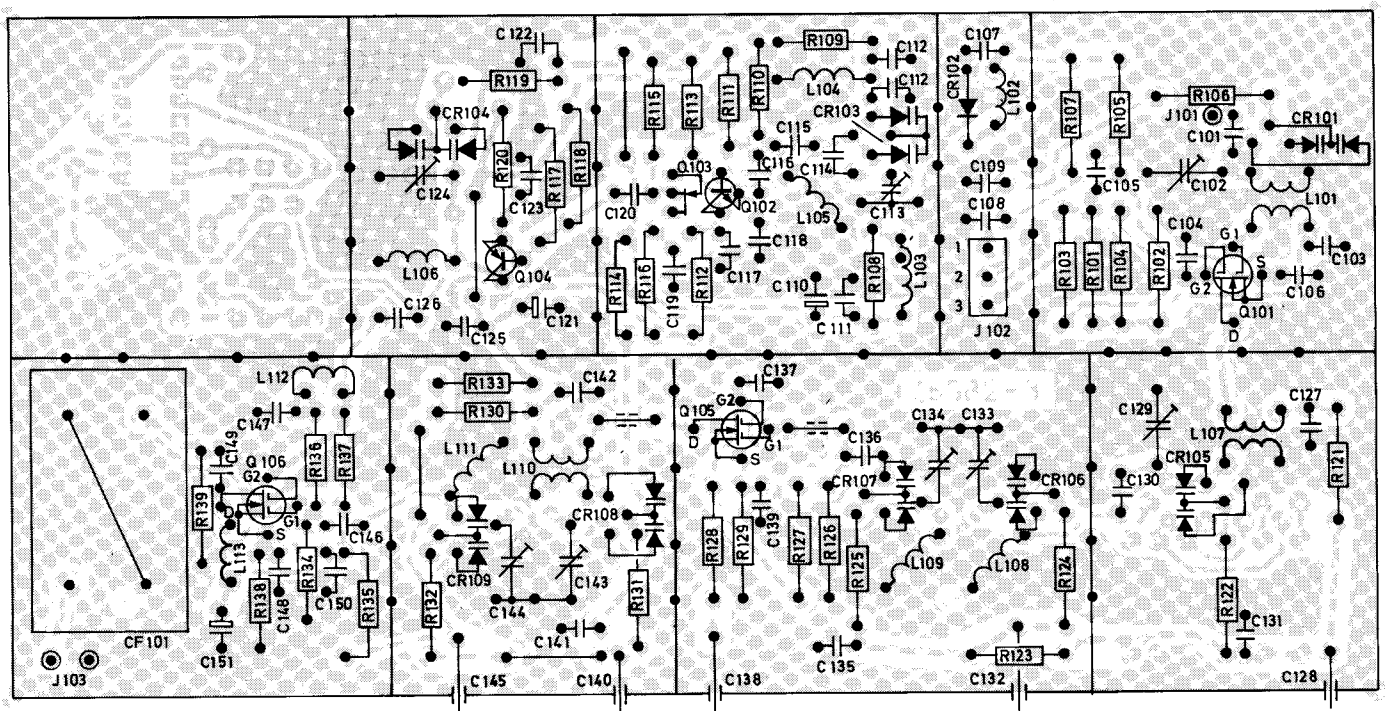
Figure 13 Front end board, foil side
