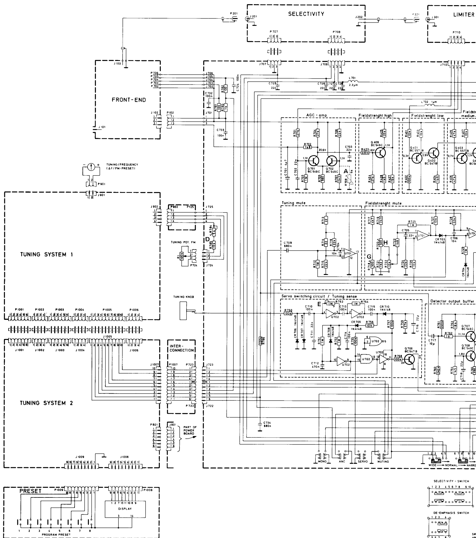
Figure 38 Main circuit diagram
