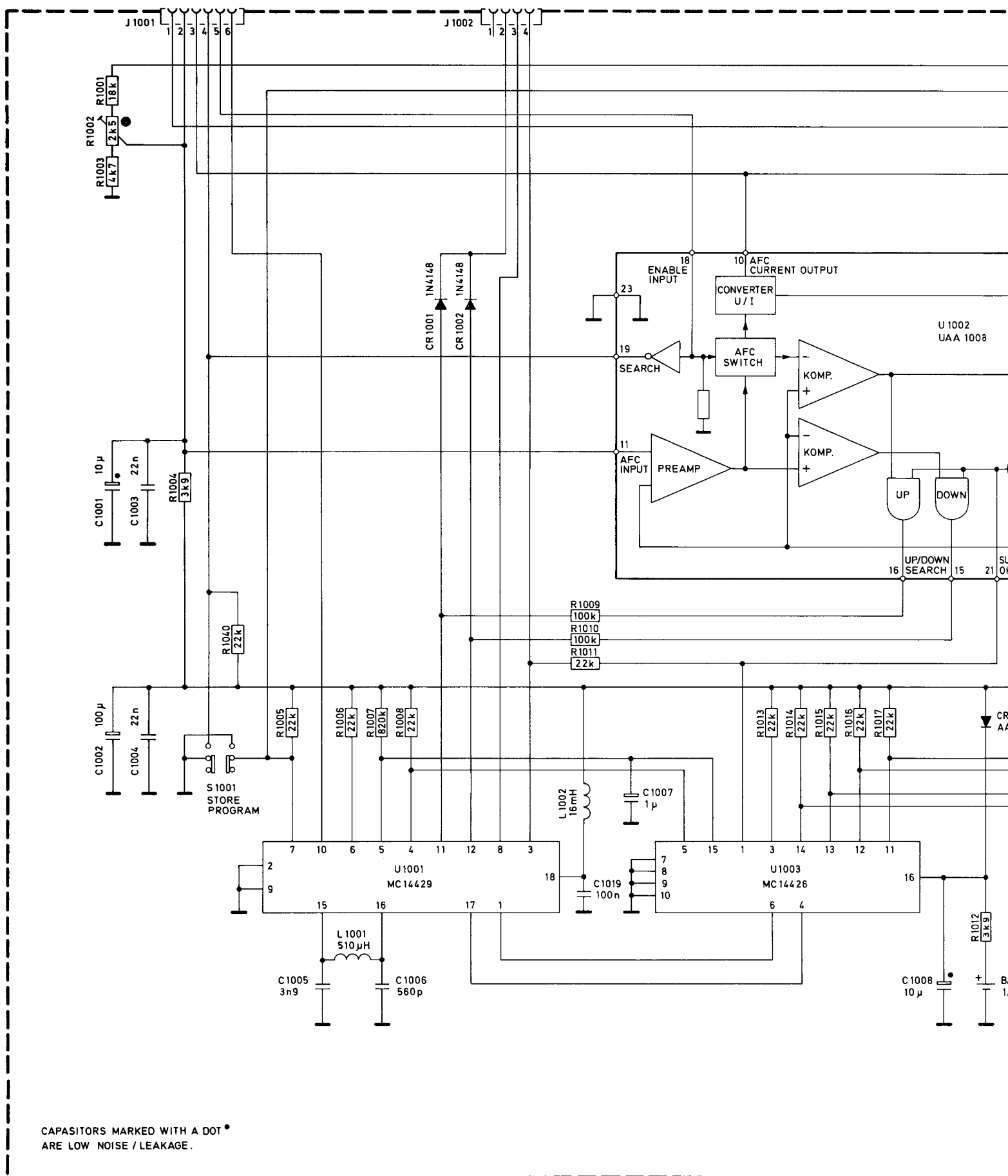
Figure 45 Tuning system 2
