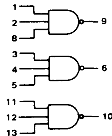
U905 MC14023
