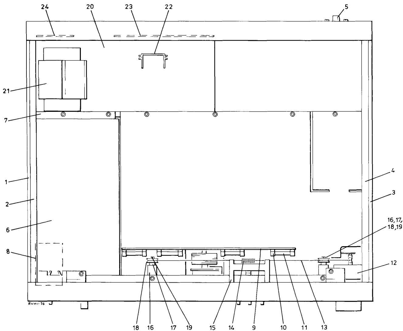
Chassis assembly - top view
