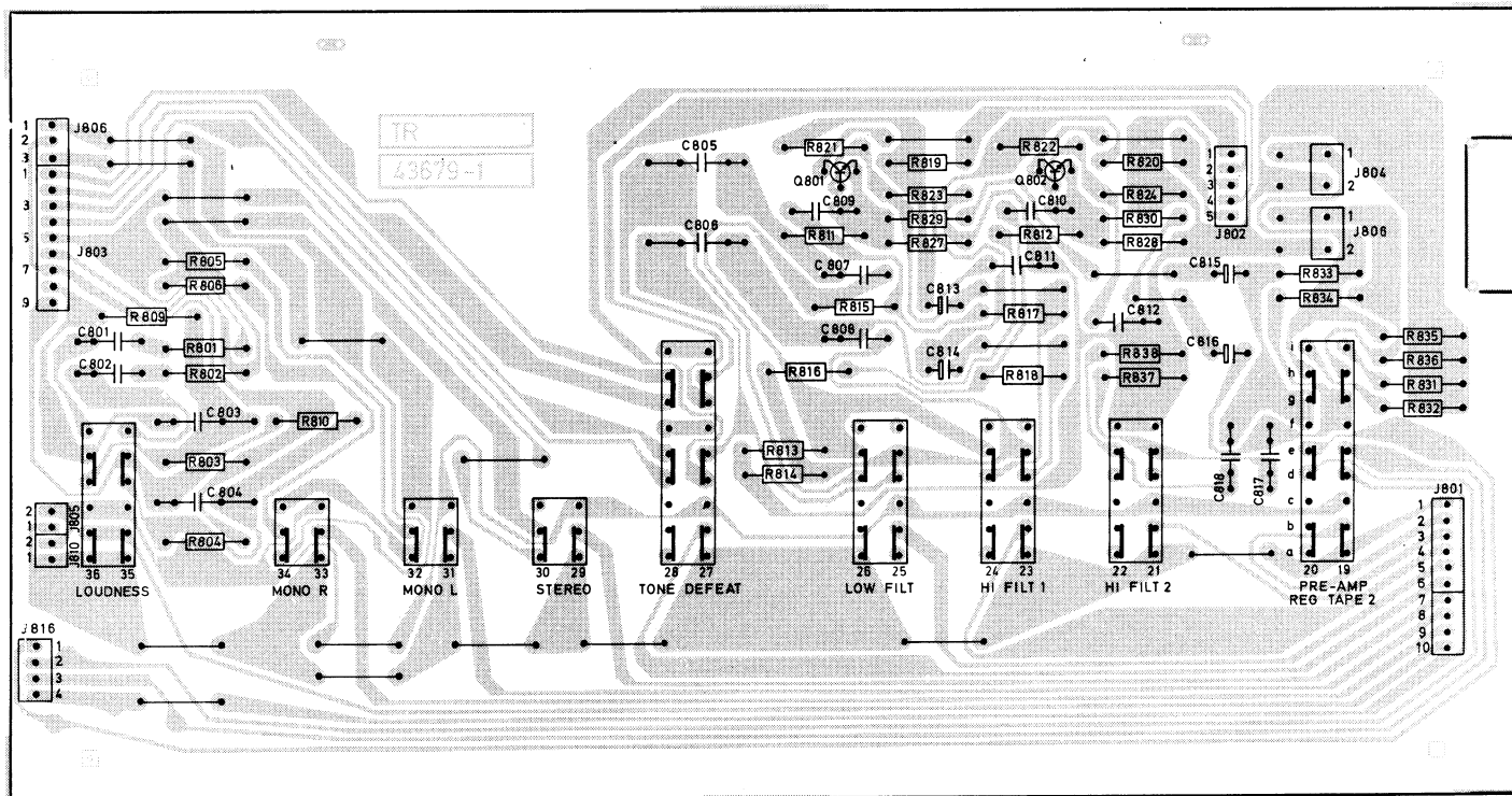
PW-BRD, MODE FILTER TL-KORT, FILTER
