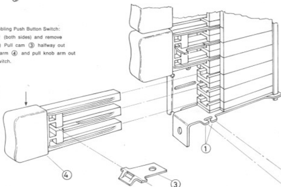
Fig. 11. Push Button assembly.
