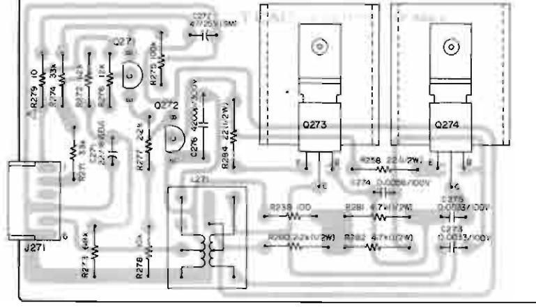
OSC PCB ASSY
