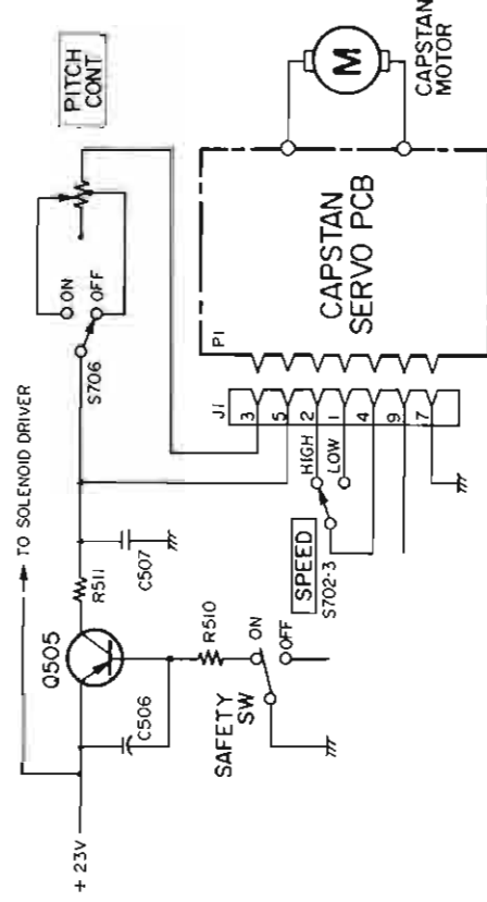
Fig. 6-3 Capstan motor circuit
