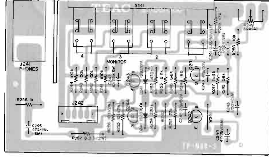
PHONE AMPL PCB ASSY
