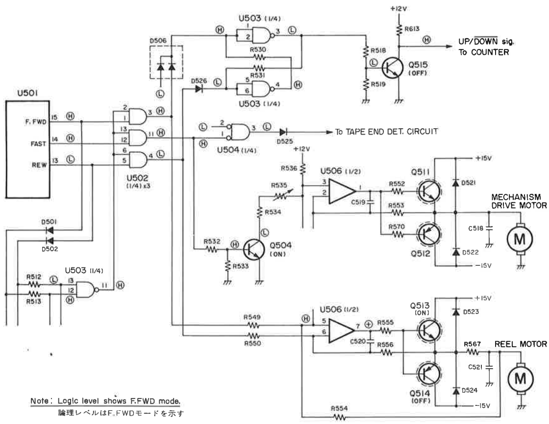
Fig. 6-6 F.FWD/REW control circuit F.FWD/REW制御回路
