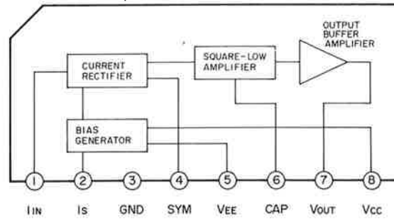
μPC1253H2 dbx NR RMS LEVEL SENSOR (TOP VIEW)
