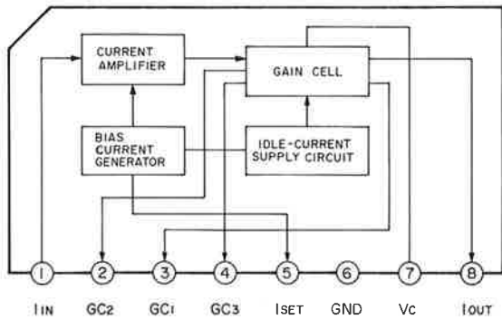
μPC1252H2 dbx NR VCA CIRCUIT (TOP VIEW)
