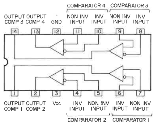
LM339N QUADRUPLE DIFFERENTIAL COMPARATOR (TOP VIEW)
