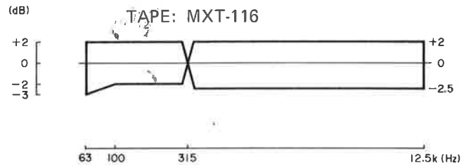
Fig. 5-10 Playback frequency response 再生周波数特性
