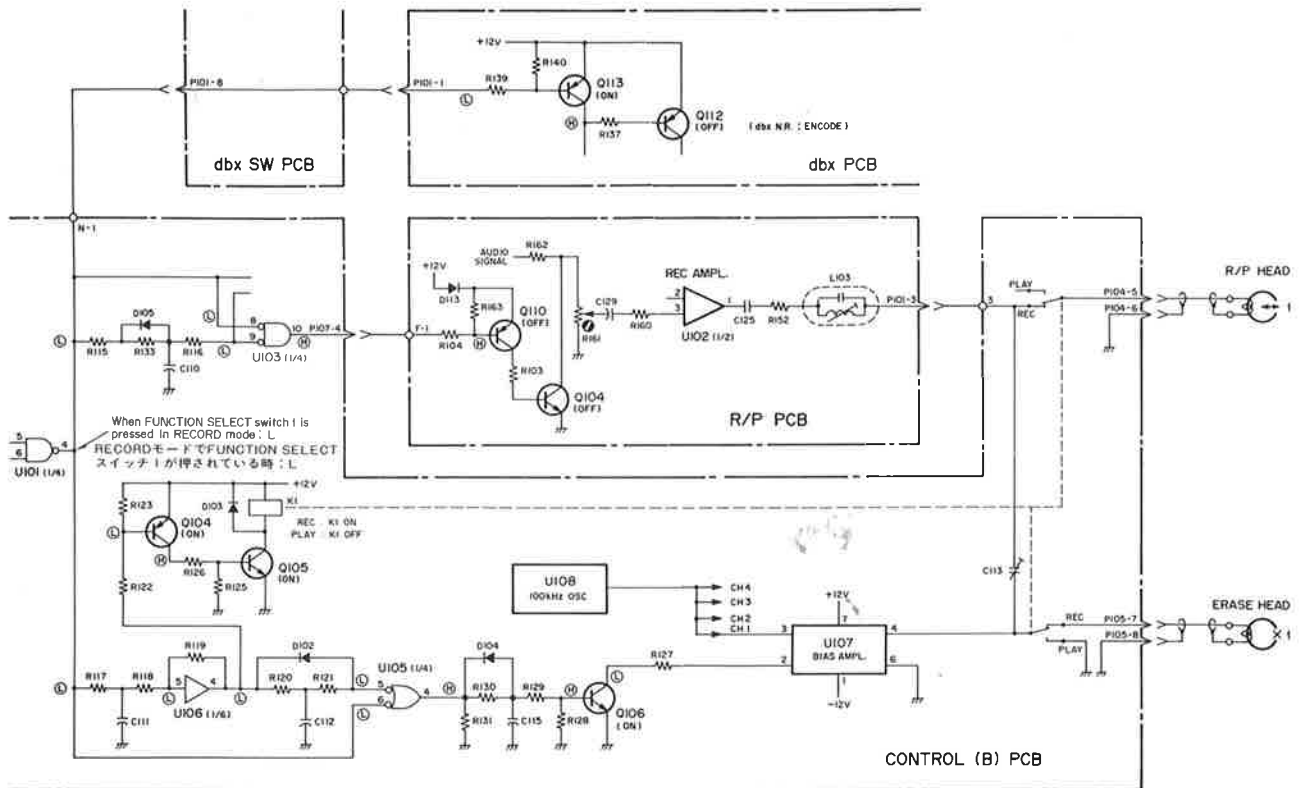
Fig. 6-16 Record control circuit 録音制御回路
