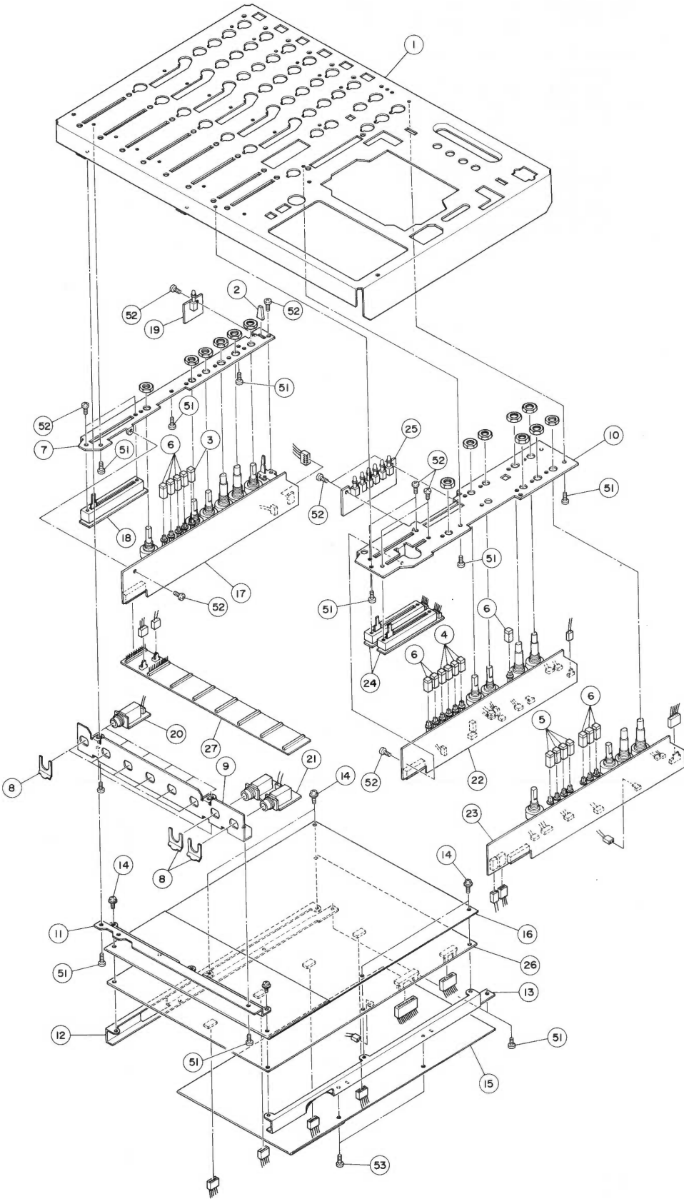
EXPLODED-VIEW-3
