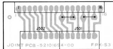
JOINT PCB ASSY
