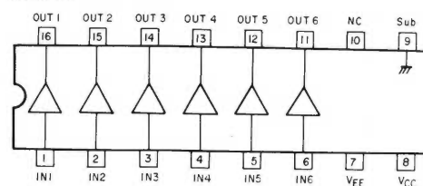
LB1294
