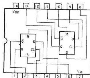
HD14013BP
