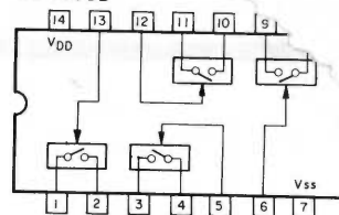
LC4066B
