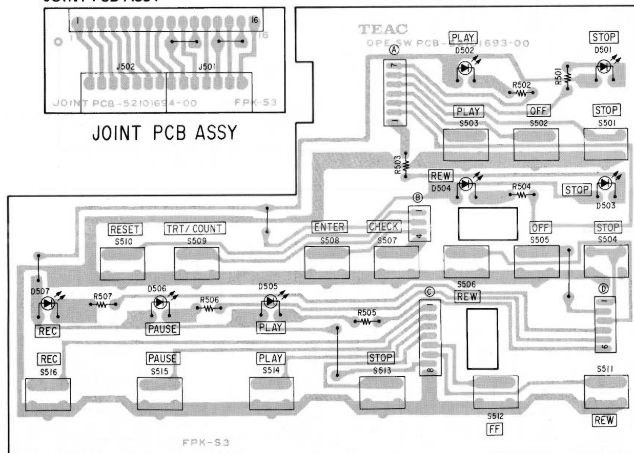
OPERATION SWITCH PCB ASSY
