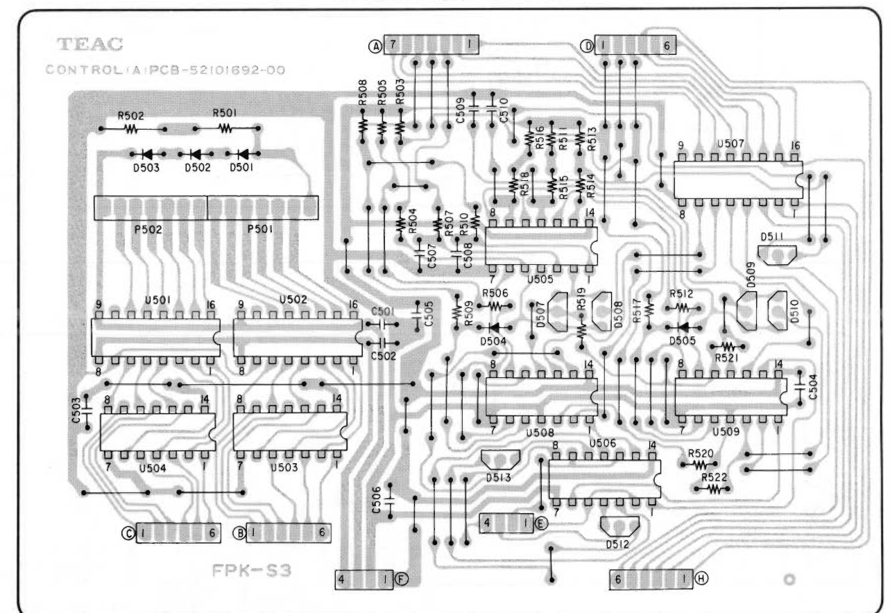
CONTROL (A) PCB ASSY
