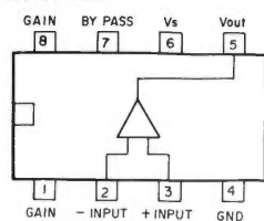
NJM386D
