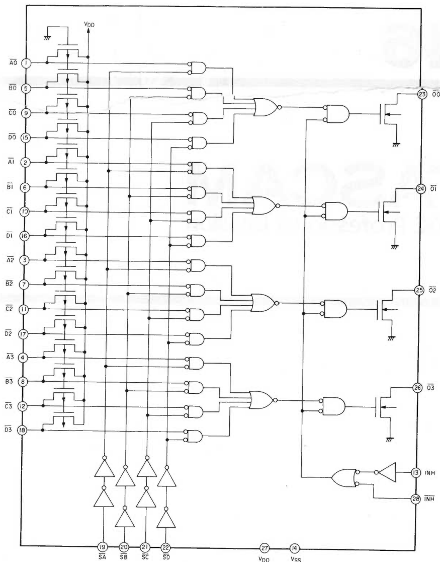
LC7800
