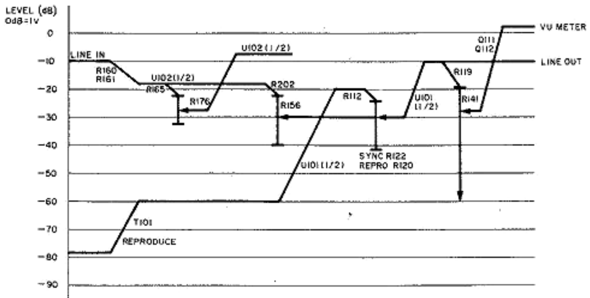
Fig. 1-17 Level Diagram
