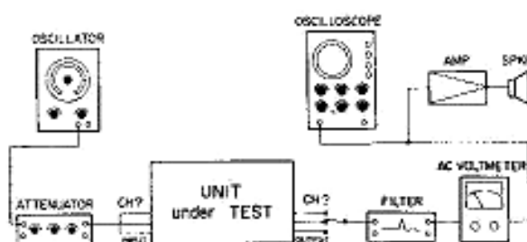
Fig. 2-18. Crosstalk Measurement Set-Up
