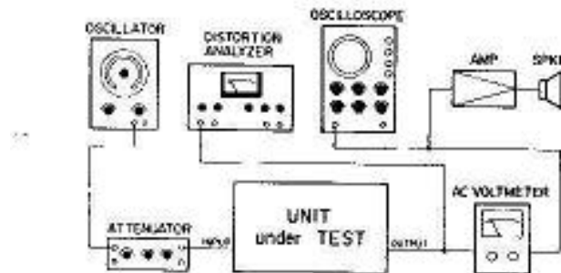
Fig. 2-19. Distortion Measurement Set-Up
