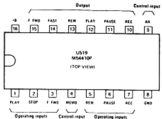
Fig. 1-1. Pin Assignments
