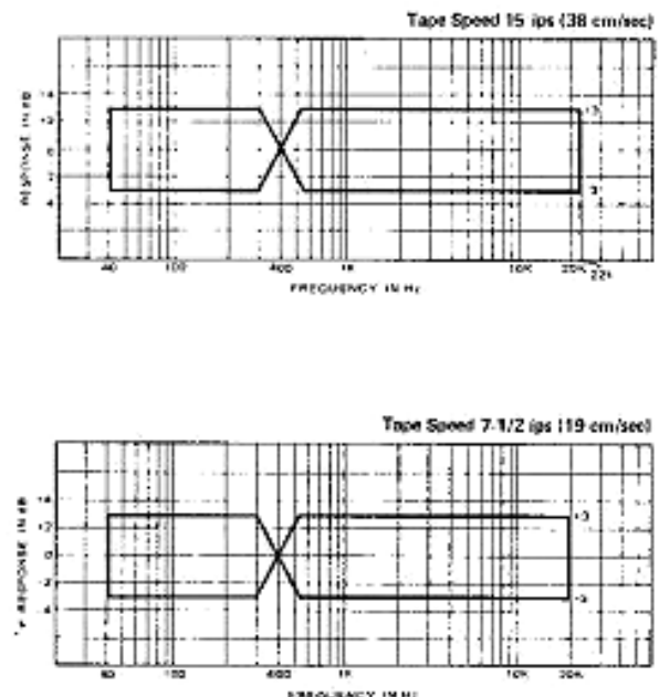
Fig. 2-16 Overall Frequency Response
