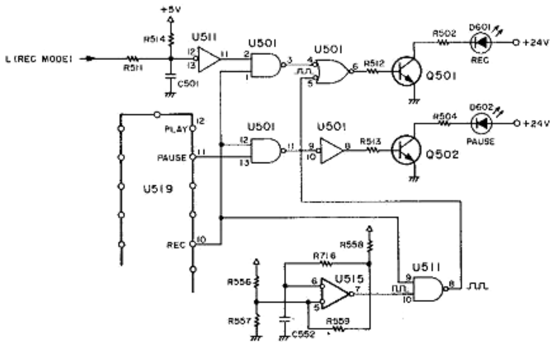
Fig. 1-13. Display Circuit
