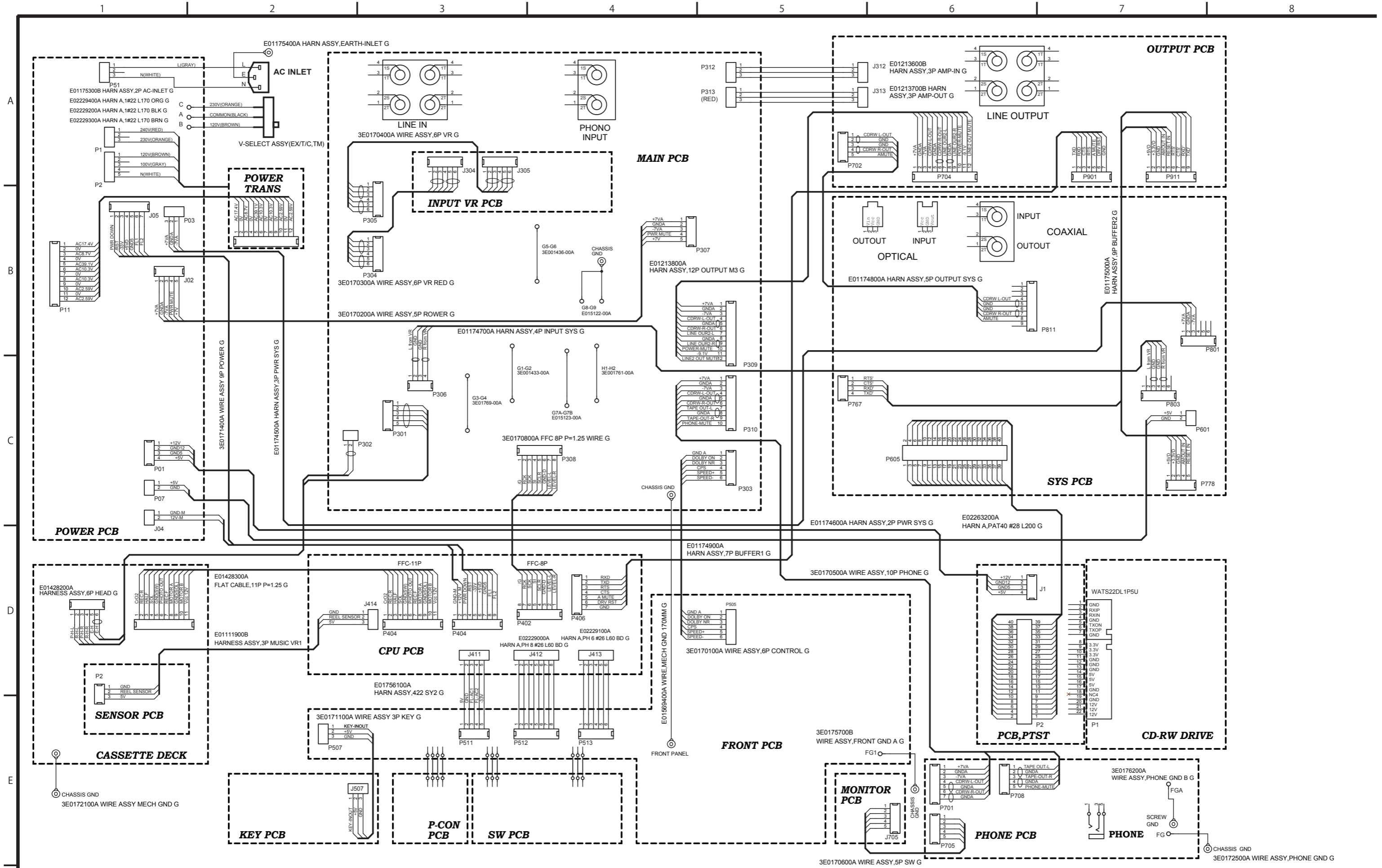
WIRING DIAGRAM
