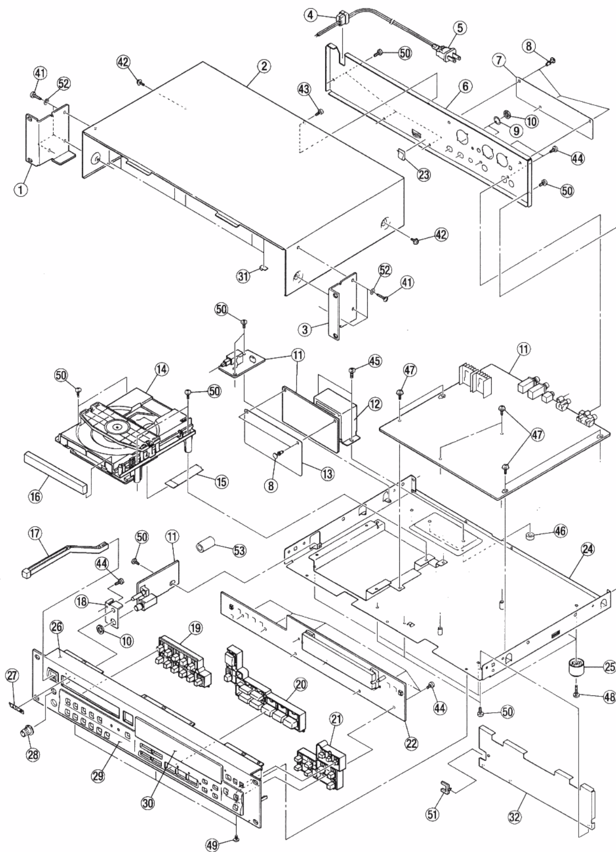
EXPLODED VIEW-1
