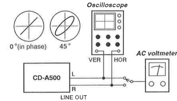
Fig. 4-4 Test setup for azimuth check
