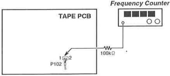
Fig. 4-7 Test setup for bias OSC adjustment
