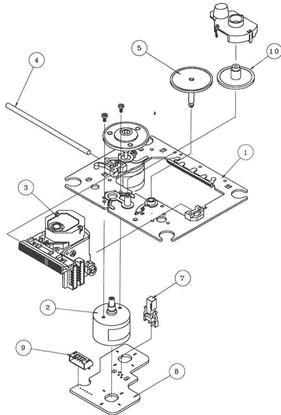
EXPLODED VIEW-4
