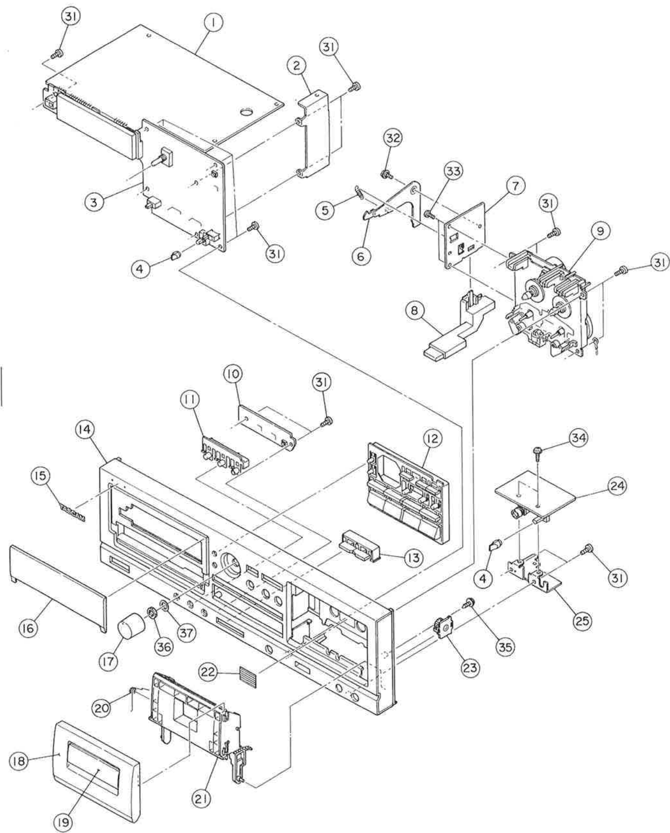
EXPLODED VIEW-2
