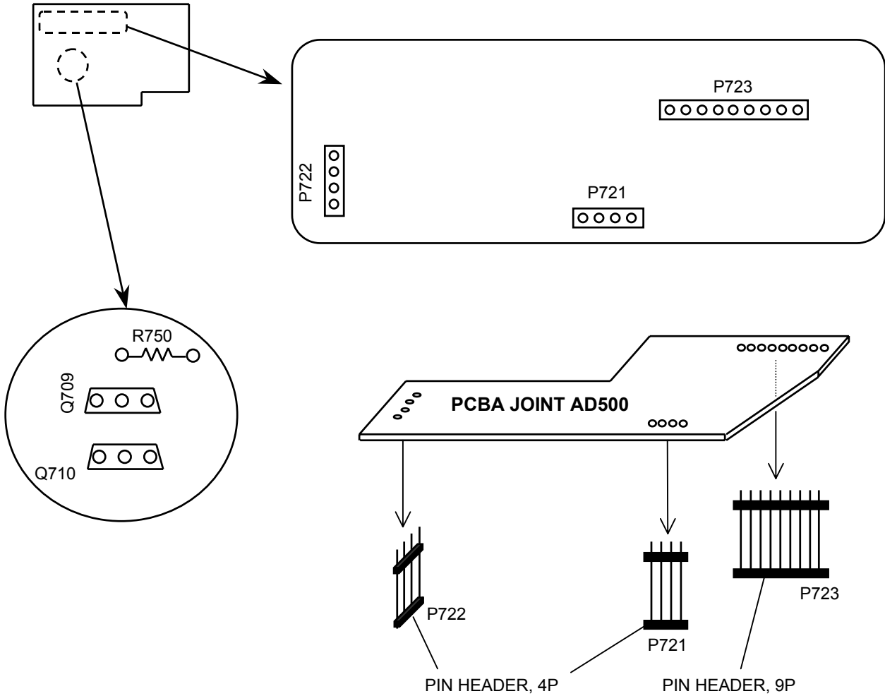
CONT-CD PCB Assy (Top View)
