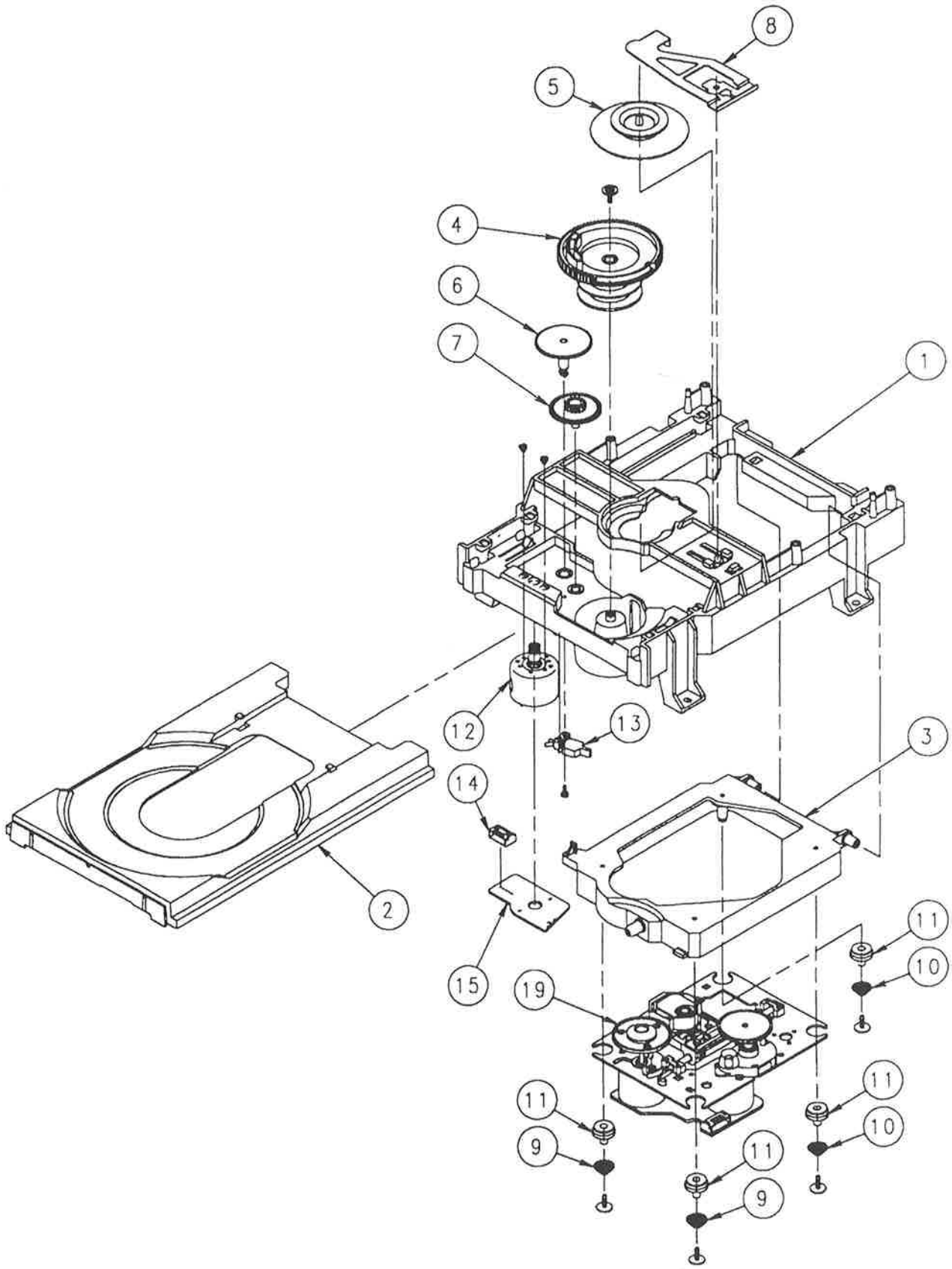
EXPLODED VIEW-3
