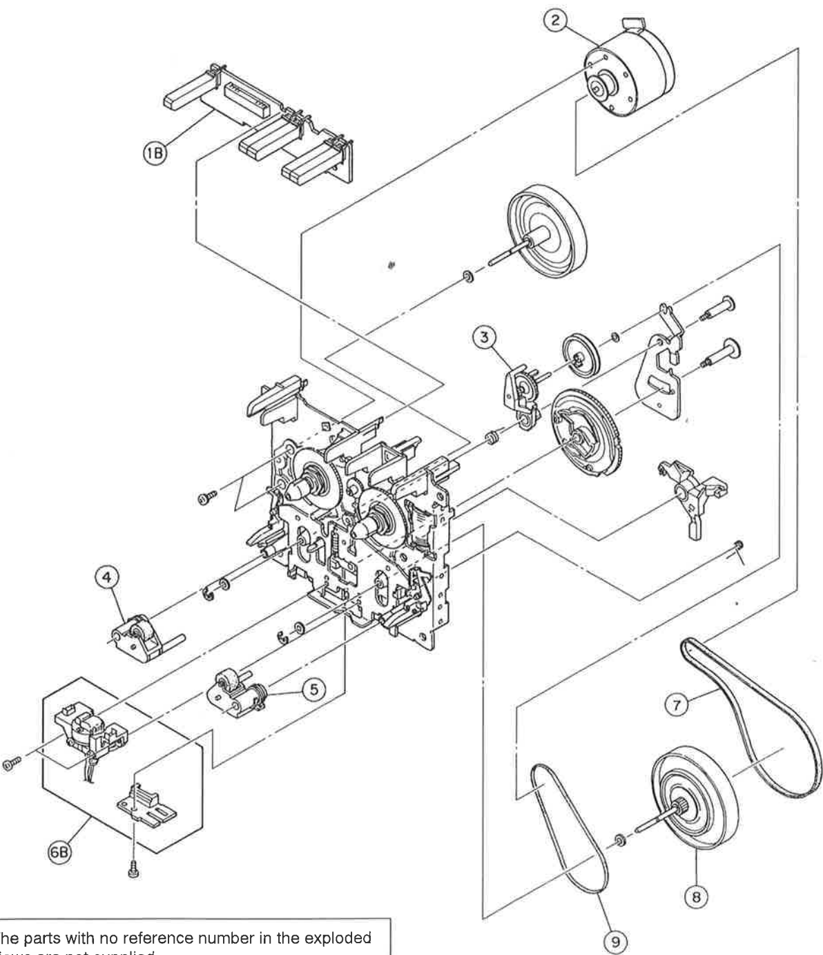
EXPLODED VIEW-5
