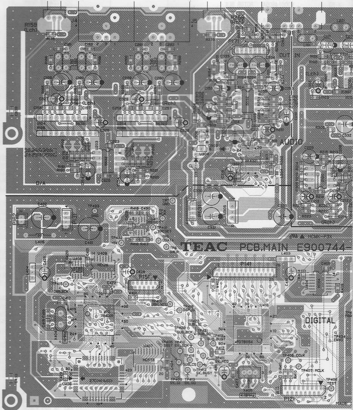
MAIN PCB
