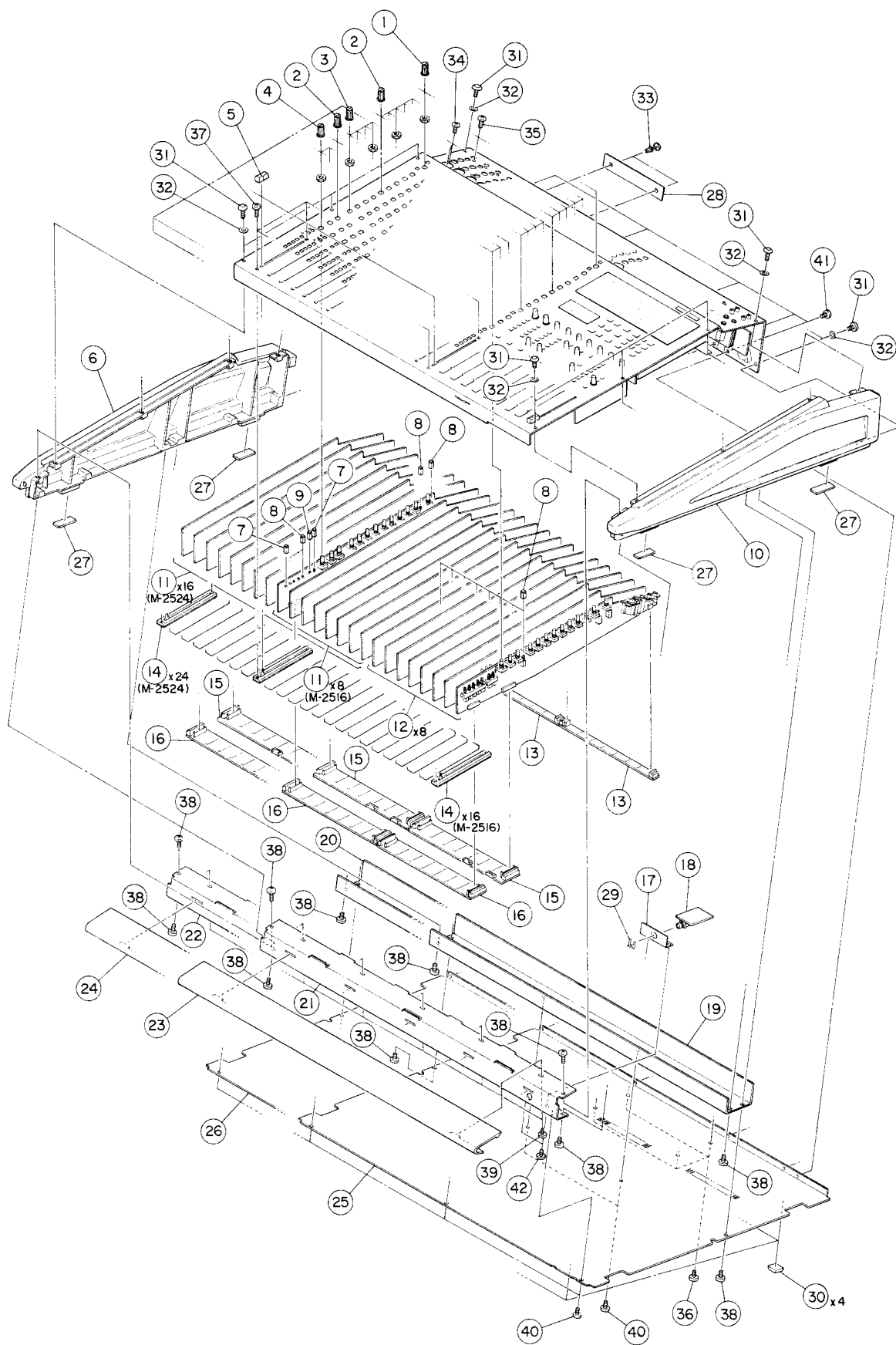
EXPLODED VIEW-1
