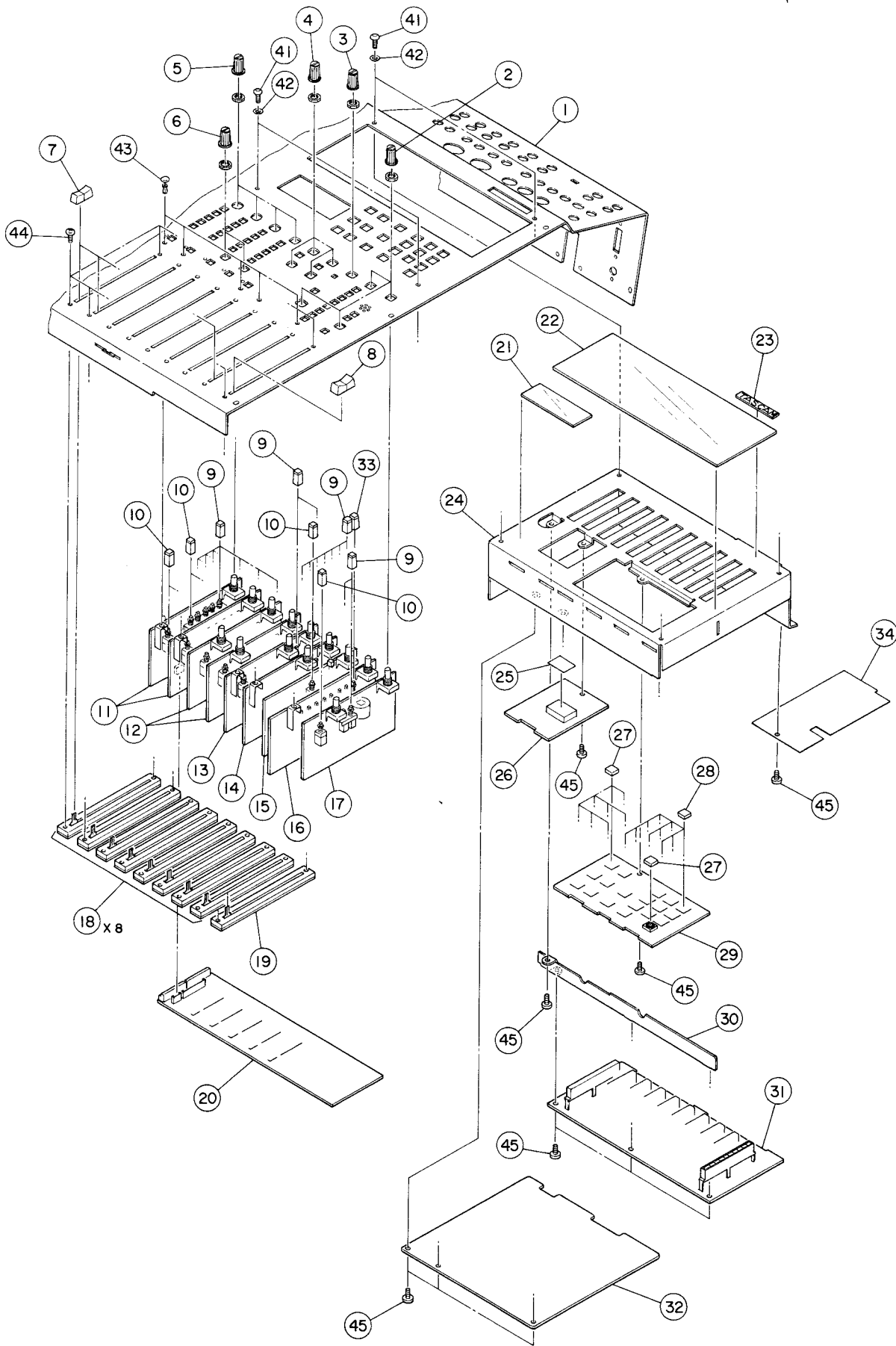
EXPLODED VIEW-3
