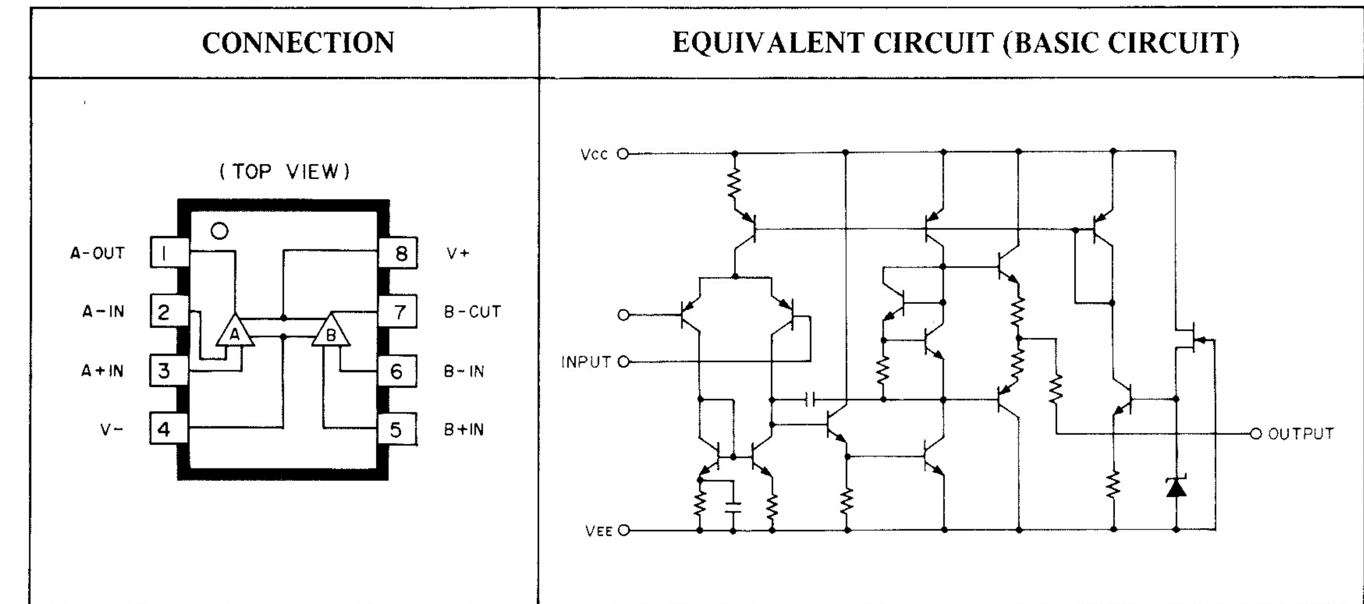
op - amp NJH4559D Dual comparator
