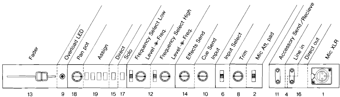
Input module layout including back panel
