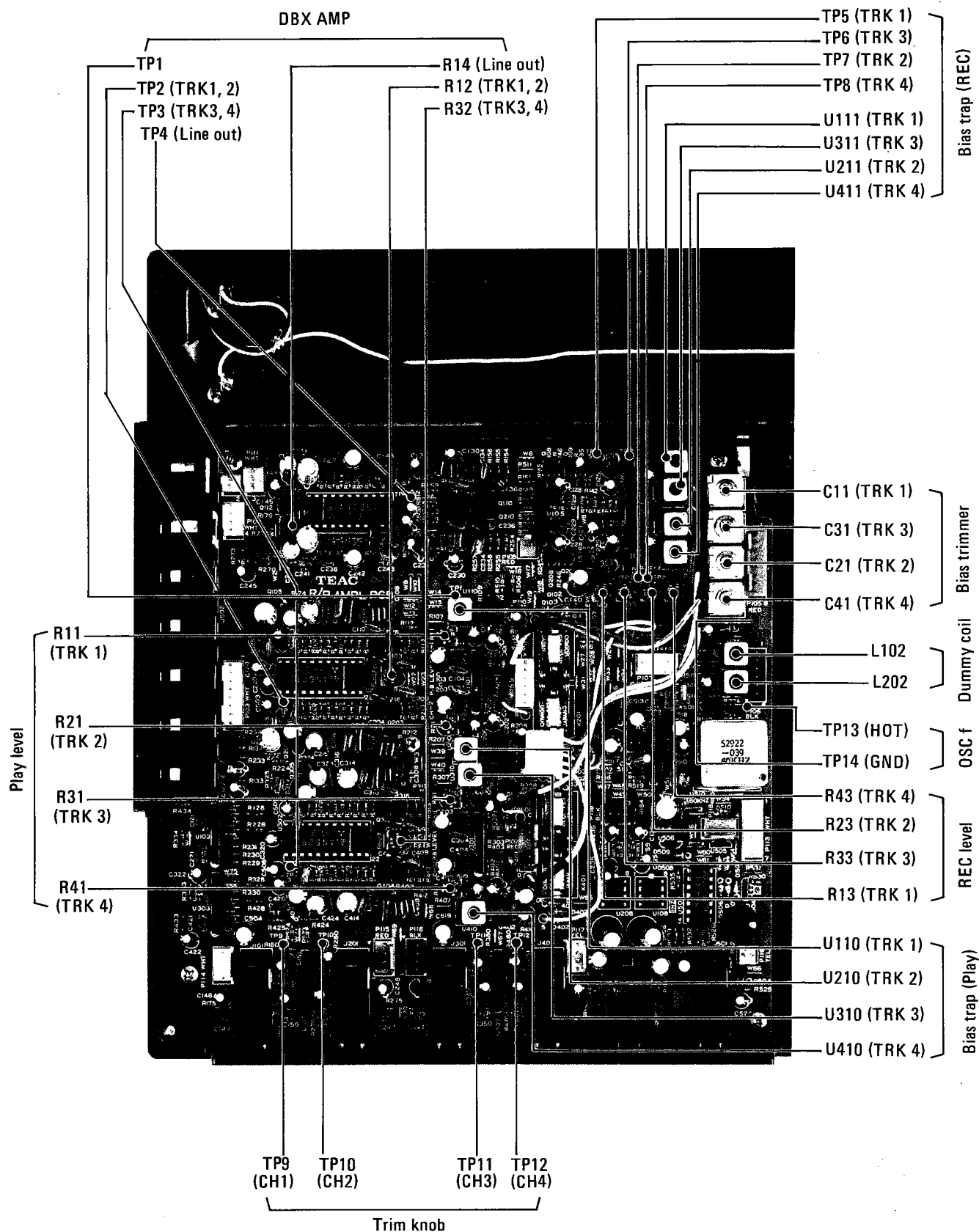
Fig. 10-1 Record/playback amplifier
