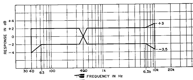
Fig. 10-4 Overall frequency response
