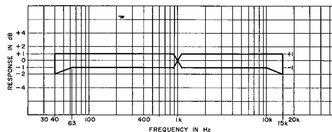
Fig. 9-3 MIC/LINE → Line out frequency response
