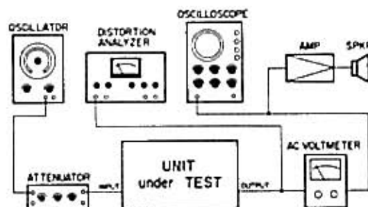
Fig. 1-5-3. Distortion Measurement Set-Up
