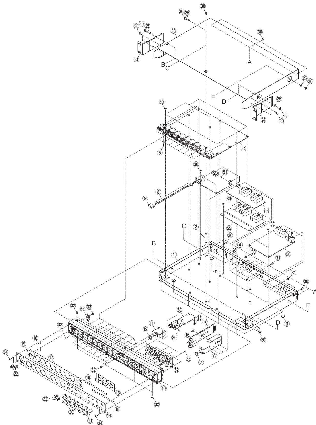
Exploded View-1
