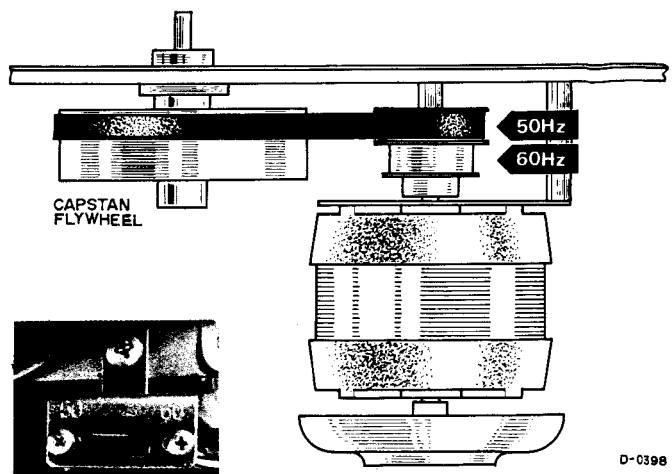
Fig. 10-2 Frequency Conversion
