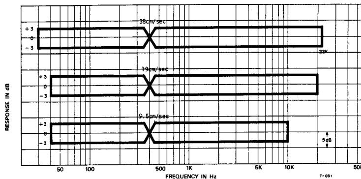
Fig. 11-2 Frequency Response -Playback-
