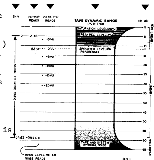
Fig. 11-7 Signal/Noise Computation
