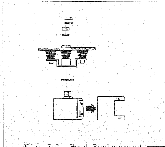
Fig. 7-1 Head Replacement
