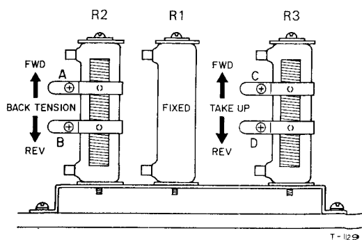
A-3300SR
