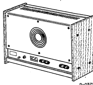
Fig. 4-1 Removing Wooden Sides
