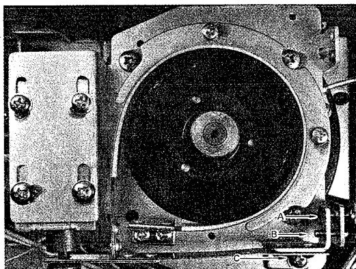
Fig. 6-4 Torque Measurement & Adjustment Location -Brake-
