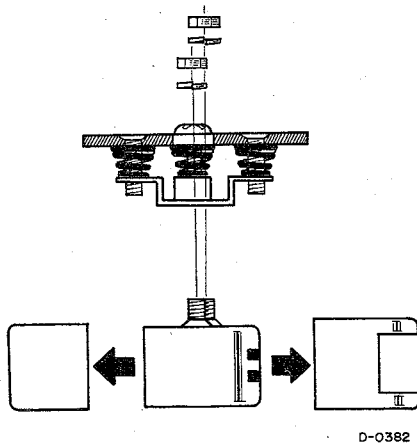
Fig. 4-4 Individual Heads
