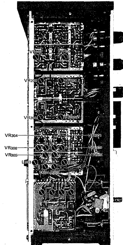
Fig. 7-1 Adjustment Locations
