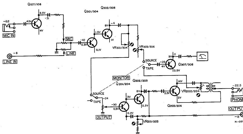
Fig. 7-5 Simplified Diagram -Monitor-
