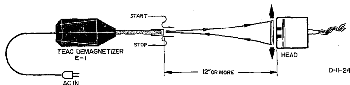
Fig. 9-2 Demagnetization
