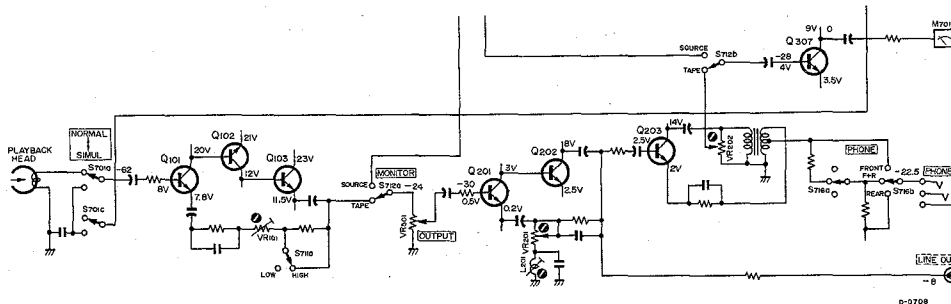
Fig. 8-2 Simplified Diagram
