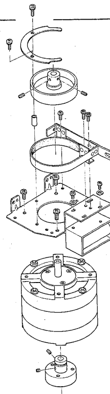
Fig. 4-8 Reel Motor Removal
