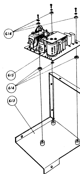
A-4000 FIG. 4 LEFT CHASSIS ASS'Y, EXPLODED VIEW
