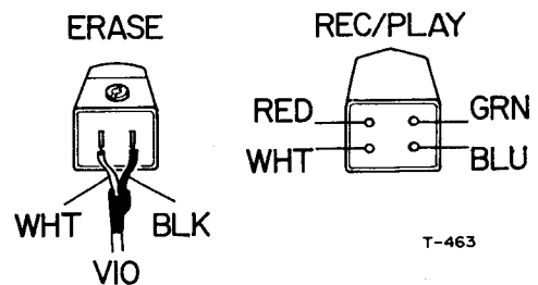
Fig. 3-5 Head Wiring Diagram
