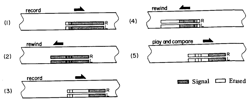
Fig. 7-19 Erase Efficiency Check Procedure
