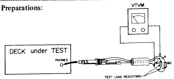
Fig. 6-8 Connection
