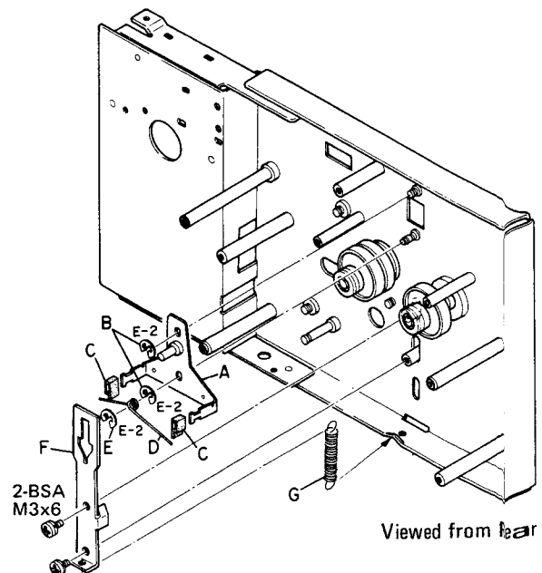
Fig. 4-9 Brake Plate Ass'y Removal
