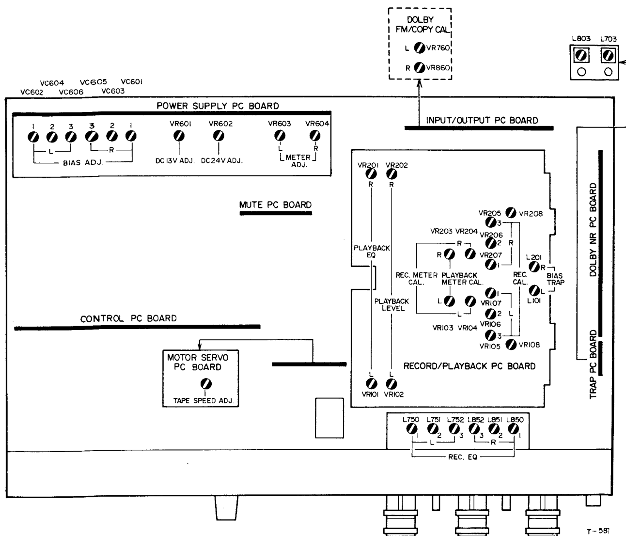
Fig. 6-1 Adjustment Location
