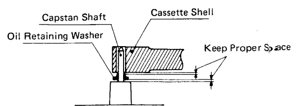
T-530 Fig. 5-14 Oil Retaining Washer Clearance Check
