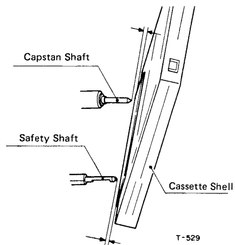
Fig. 5-13 Cassette Holder Motion Checks T-529
