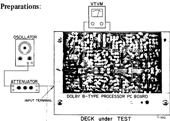
Fig. 6-9 Connection
