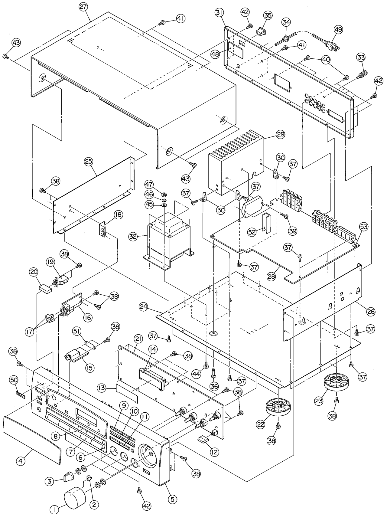
EXPLODED VIEW-1
